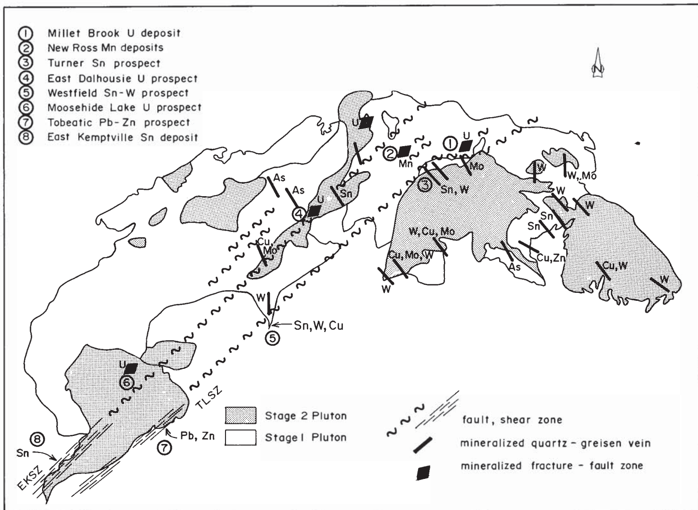
Fig. 11. Map showing the distribution of mineralized NW-trending quartz-grisen veins and NE-trending faults and associated fractures within South Mountain Batholith.
