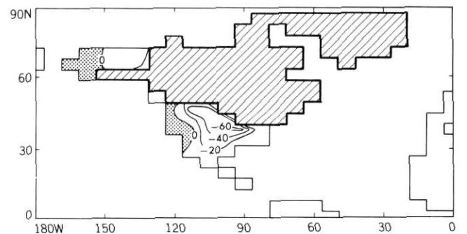
FIGURE 6. Percentage change in annual mean soil moisture from the control to the ice sheet experiment. Areas covered by continental ice are hatched; areas of positive soil moisture change are stippled.
