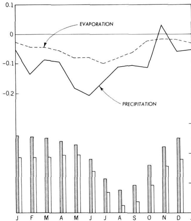
FIGURE 7. Seasonal variations in area-averaged soil moisture (cm) for the dry zone that develops south of the Laurentide Ice Sheet from the ice sheet and control experiments. The vertical bars indicate the monthly mean soil moisture, with the stippled and open bars representing the control and ice sheet experiments, respectively. Differences in precipitation and evaporation (including sublimation) between the two experiments (cm/d) are shown by solid and dashed lines, respectively.
