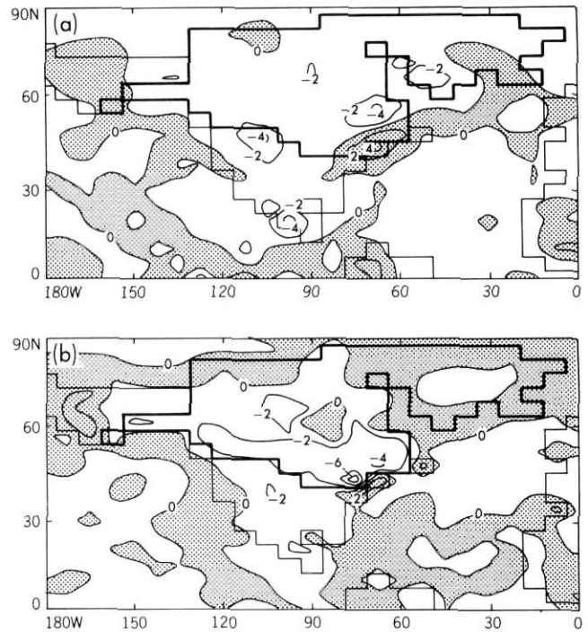
FIGURE 8. Differences in precipitation (top) and evaporation including sublimation (bottom) between the ice sheet and control experiments for the summer season. The heavy solid outline indicates the continental ice boundary. Units are mm/d.
