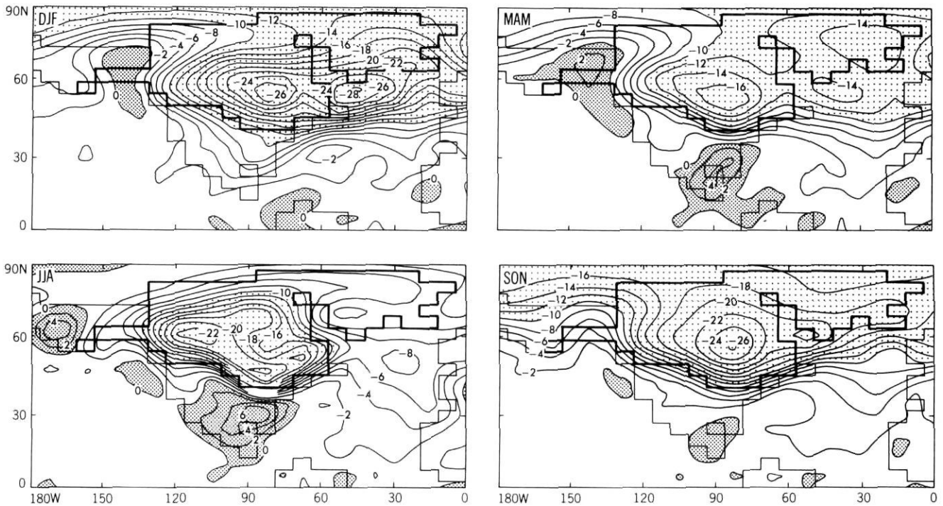
FIGURE 5. Difference in surface air temperature between the ice sheet and control experiments for each season ( ^{\circ}\text{C} ). Areas of temperature increase are densely stippled, while areas of temperature decrease greater than 10^{\circ} are lightly stippled. The heavy solid outline indicates the continental ice boundary.
