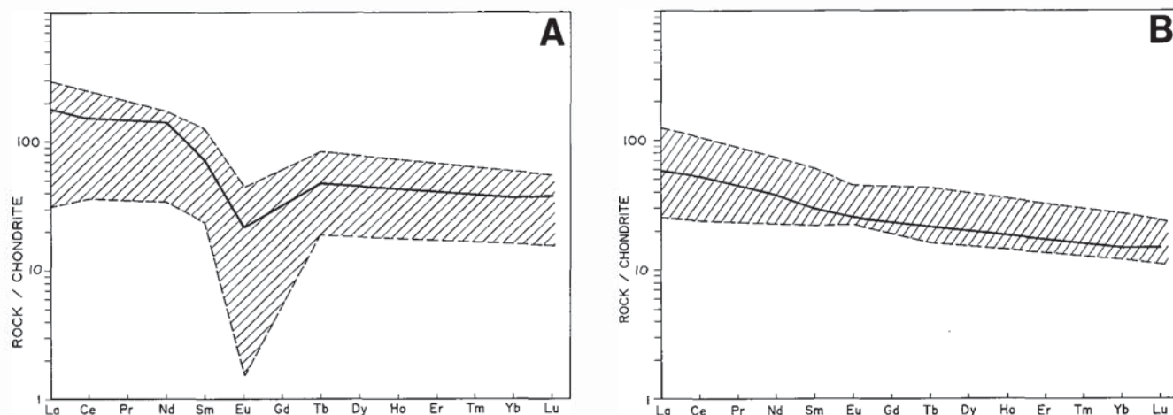
Fig. 8. Average chondrite-normalized REE profiles (solid lines) and range of values (cross-hatched) in volcanic rocks of the Riley Brook area. (A) felsic volcanic rocks ( n=8 ); (B) mafic volcanic rocks ( n=8 ). Normalizing values after Frey et al. (1968).
