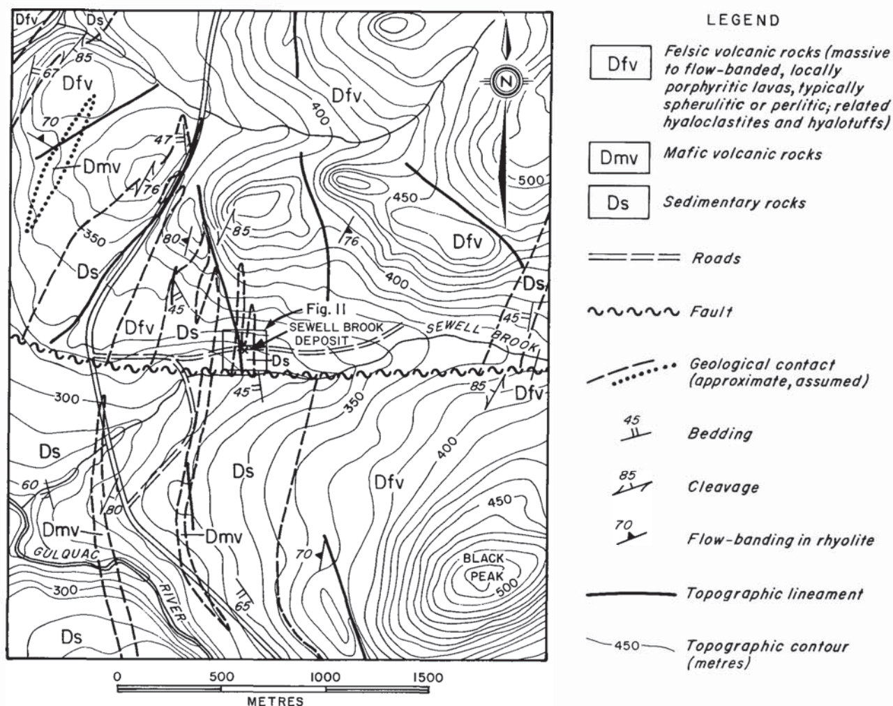
Fig. 10. Local geology of the Sewell Brook area.
