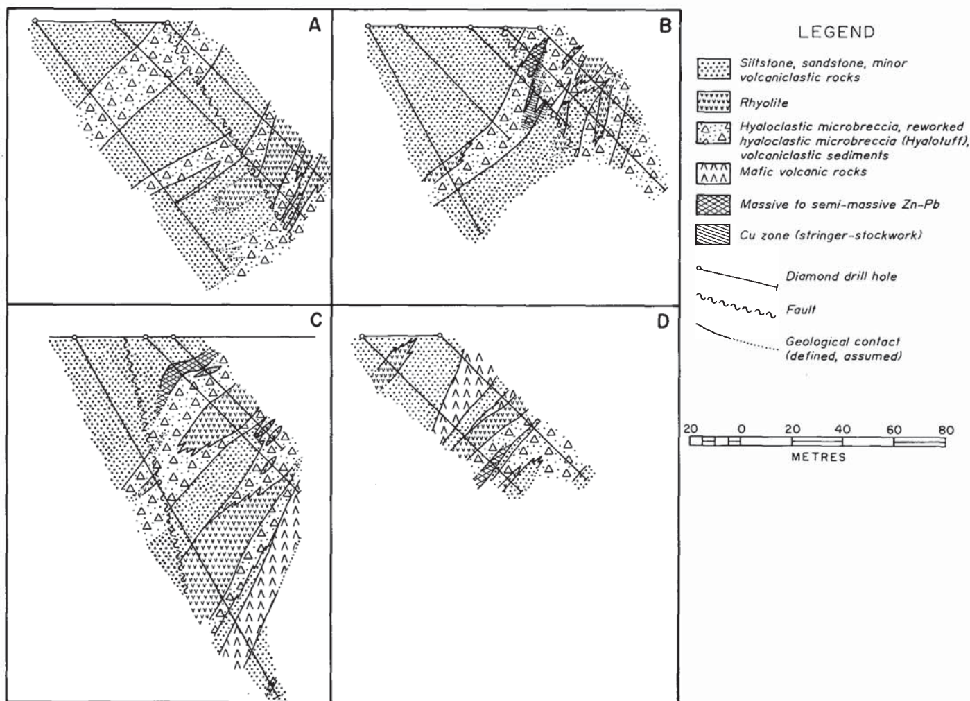
Fig. 12. Cross-sections showing simplified geology of the Sewell Brook deposit.
