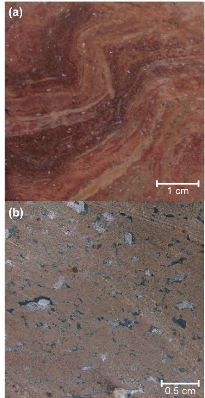
Fig. 3. Slab photographs indicating (a) flow-banded rhyolite with a quartzofeldspathic groundmass, and (b) vuggy trachyte with chlorite infillings.
