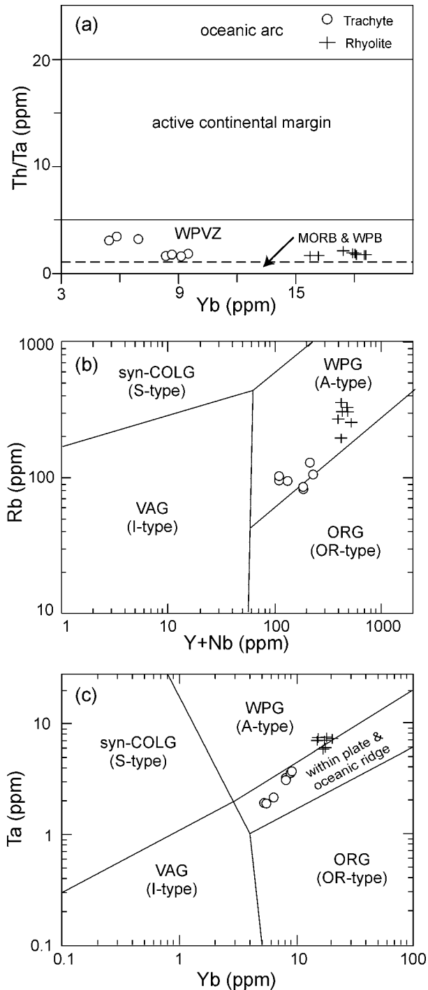
Fig. 8. Discrimination diagrams for felsic volcanic rocks from the Cumberland Hill Formation. (a) Yb (ppm) versus Th/Ta (Gorton and Schandl 2000). Abbreviations: WPVZ = within plate volcanic zones; MORB = mid-ocean ridge basalt; WPB = within-plate basalt. (b) Rb vs Nb + Y and (c) Ta vs Yb (Pearce et al. 1984). Abbreviations: syn-COLG = syn-collisional granite; WPG = within-plate granite; VAG = volcanic-arc granite; ORG = oceanic-ridge granite.
