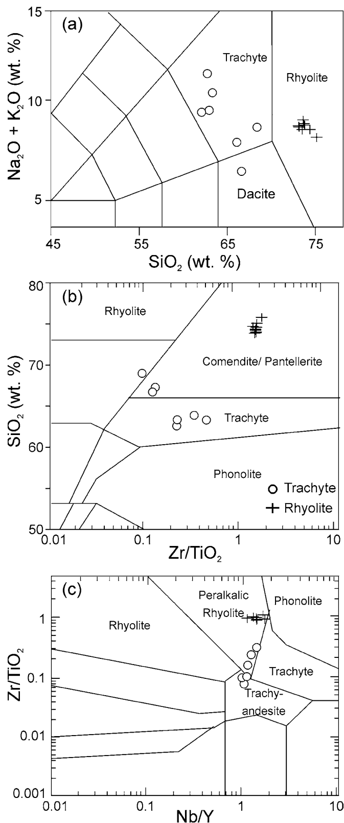
Fig. 4. Plots of (a) Na_2O + K_2O versus SiO_2 (wt. %; Le Maitre et al. 1989); (b) SiO_2 versus Zr/TiO_2 (wt. %; Winchester and Floyd 1977); and (c) Zr/TiO_2 versus Nb/Y (Winchester and Floyd 1977) for volcanic samples from the Cumberland Hill Formation.
