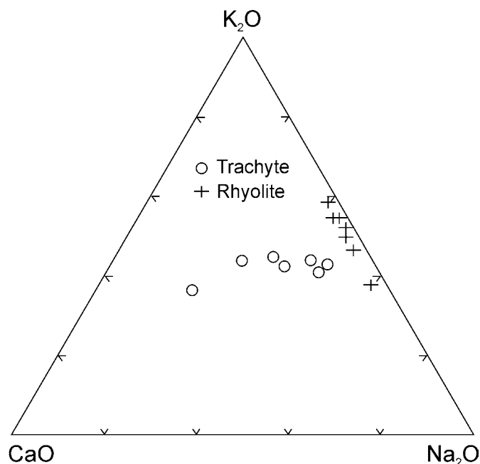
Fig. 6. CaO-K 2 O-Na 2 O ternary diagram for volcanic samples from the Cumberland Hill Formation. Trends indicate that fractionation of Ca-plagioclase and clinopyroxene could have occurred in trachyte, whereas alkali feldspar fractionation is more likely in rhyolite.
