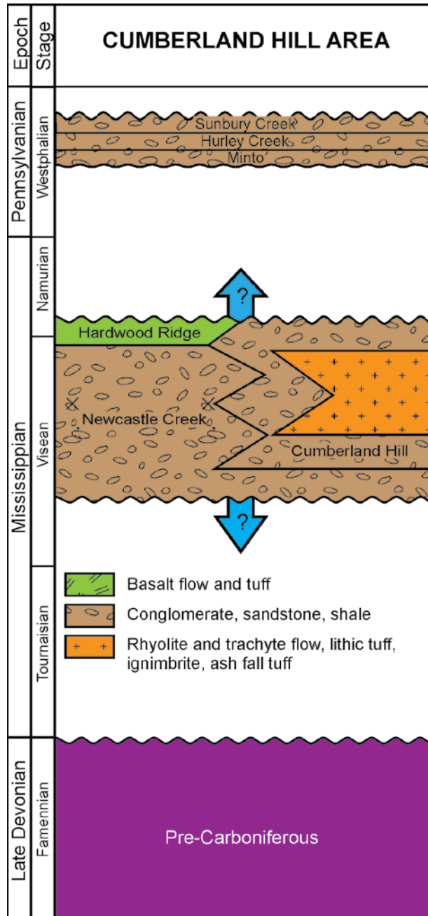
Fig. 2. Carboniferous stratigraphy in the central New Brunswick Basin (adapted from St. Peter 1997). The Cumberland Hill and Hardwood Ridge formations are part of the Mabou Group, whereas the Minto Formation, Hurley Creek Formation and Sunbury Creek Formation belong to the Pictou Group.
