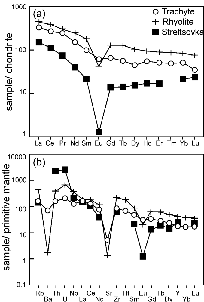
Fig. 7. (a) Chondrite-normalized REE patterns of the averages of trachyte ( n = 7 ) and rhyolite ( n = 8 ) samples from the Cumberland Hill Formation and rhyolite from Streltsovka ( n = 1 ; Chabiron et al. 2003); (b) Primitive mantle-normalized multi-element plots of the average of trachyte ( n = 7 ) and rhyolite ( n = 8 ) samples from the Cumberland Hill Formation and rhyolite from Streltsovka ( n = 1 ; Chabiron et al. 2003). Normalizing values are after Sun and McDonough (1989).
