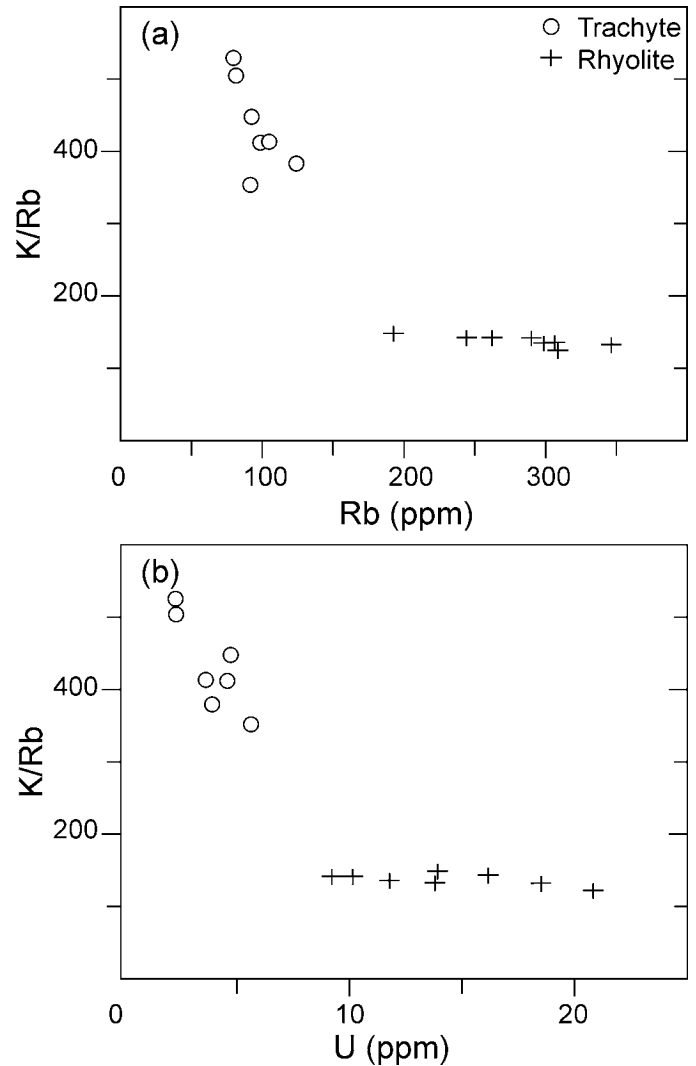
Fig. 9. Plot of K/Rb versus (a) Rb (ppm) and (b) U (ppm) in felsic volcanic samples from the Cumberland Hill Formation.
