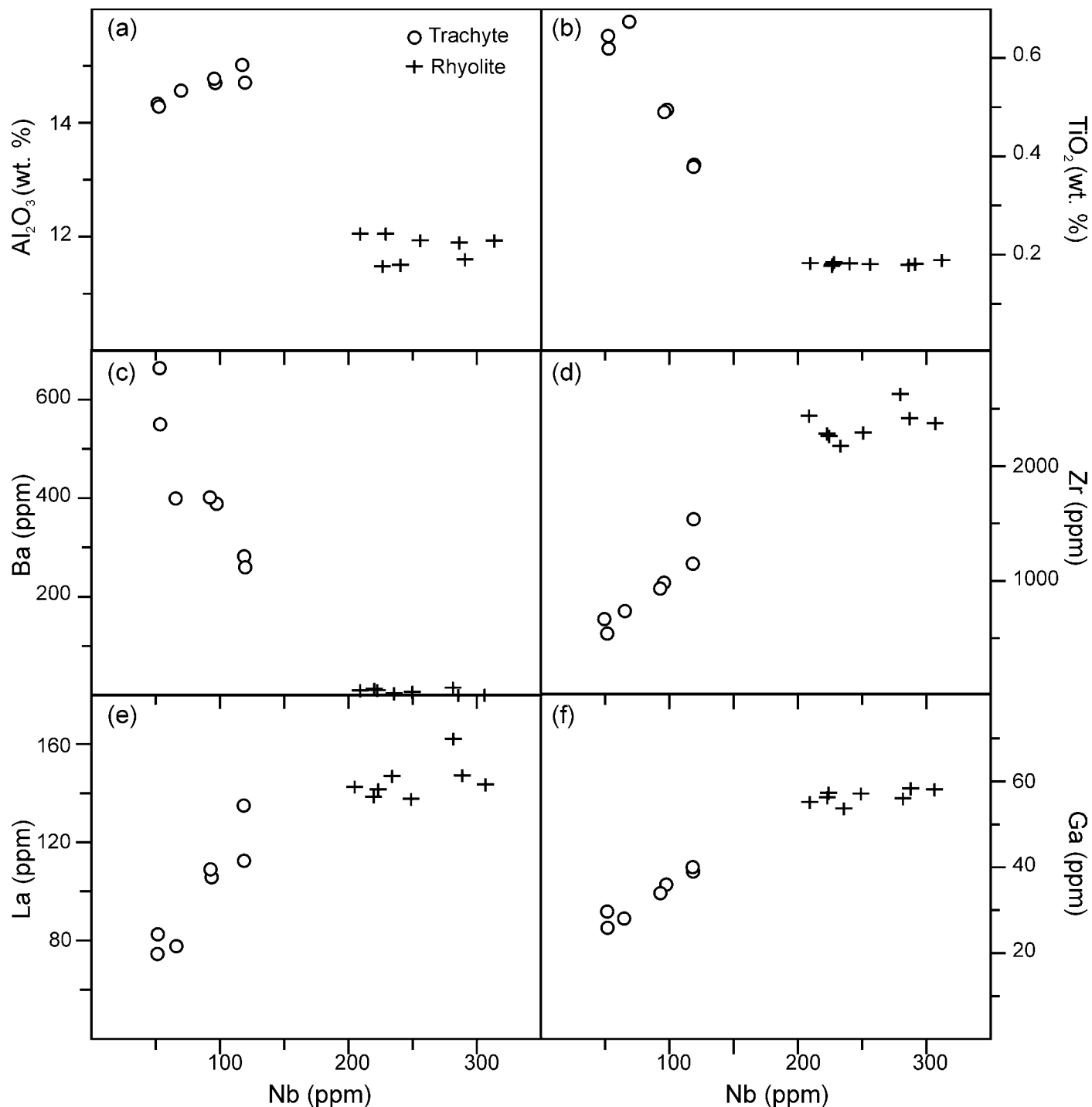
Fig. 5. Plots of Nb (ppm) versus (a) \text{Al}_2\text{O}_3 (wt. %), (b) \text{TiO}_2 (wt. %), (c) Ba (ppm), (d) Zr (ppm), (e) La (ppm), and (f) Ga (ppm) for volcanic samples from the Cumberland Hill Formation.
