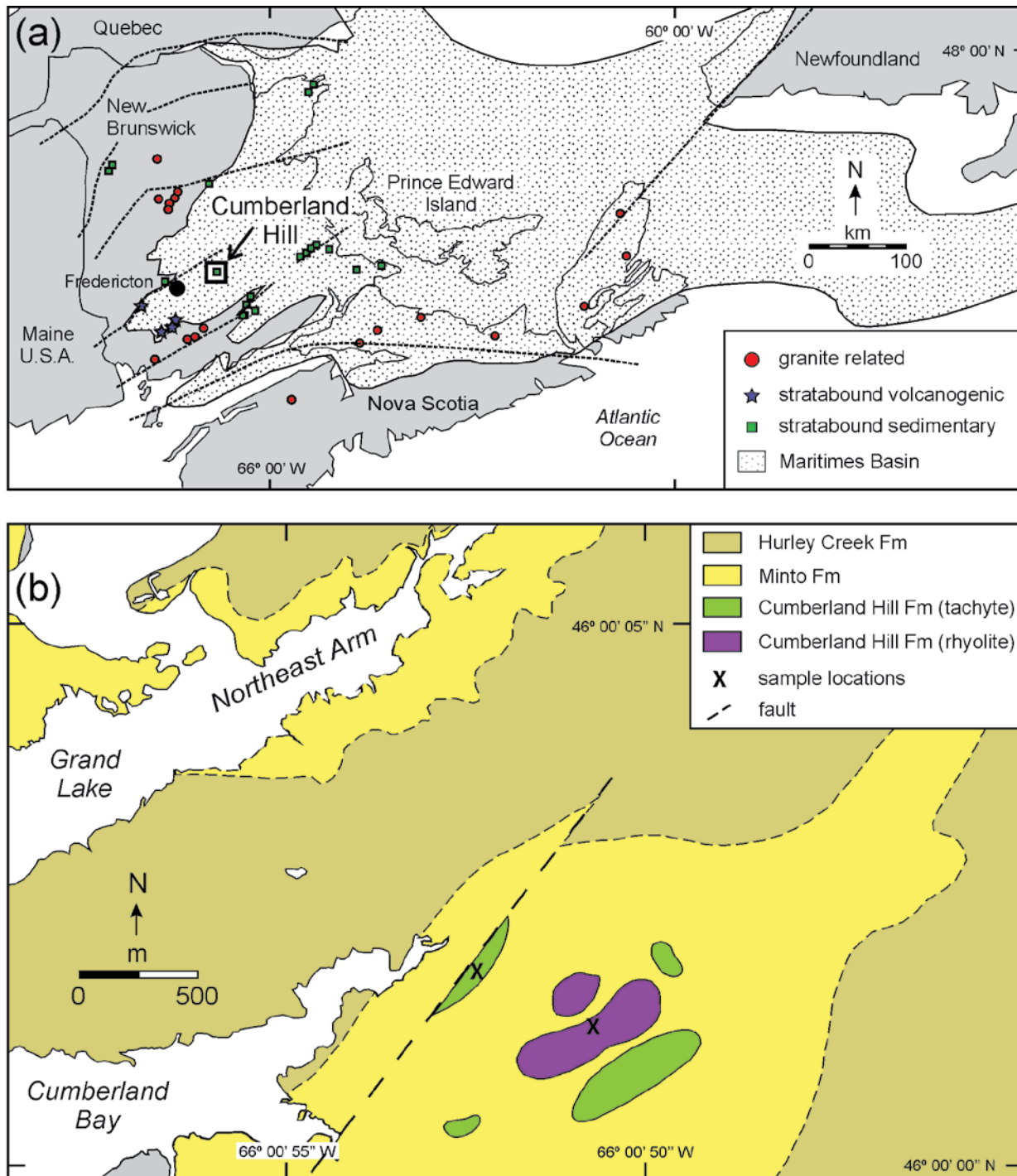
Fig. 1. (a) Map of Atlantic Canada depicting the Maritimes Basin, adapted from Roliff (1962), Williams (1974), Bradley (1982), and Fyffe and Barr (1986). Major faults are indicated as dashed lines; study area is indicated with a box. Red circles, blue stars and green squares represent different types of uranium occurrences within the Maritimes Basin (McLeod and Smith 2010; Dostal et al. 1983); (b) Geological map of the Cumberland Hill area, southern New Brunswick (adapted from Smith 2007) indicating the areal extent of the Cumberland Hill trachyte and rhyolite, both of which are interbedded with lithic and feldspathic sandstone and conglomerate, and contain interdigitating feldspar porphyry, rhyolite ash tuff, breccia, and lapilli tuff (New Brunswick Department of Natural Resources 2010a). The Hurley Creek Formation is composed of mudstone, fine-grained sandstone, coarse-grained feldspathic and lithic sandstone and polymictic pebble conglomerate at the top (Muller 1951). The Minto Formation contains feldspathic, pebbly and fine-grained sandstone, polymictic conglomerate and minor laminated mudstone, shale and thin coal seams (Dyer 1926; Muller 1951; St. Peter 2000).
