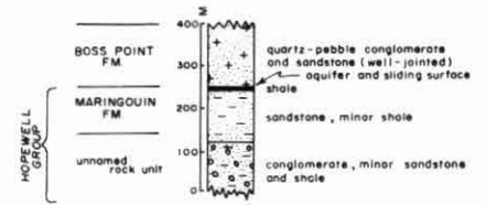
Figure 2 Stratigraphic column, Herring Cove area.
