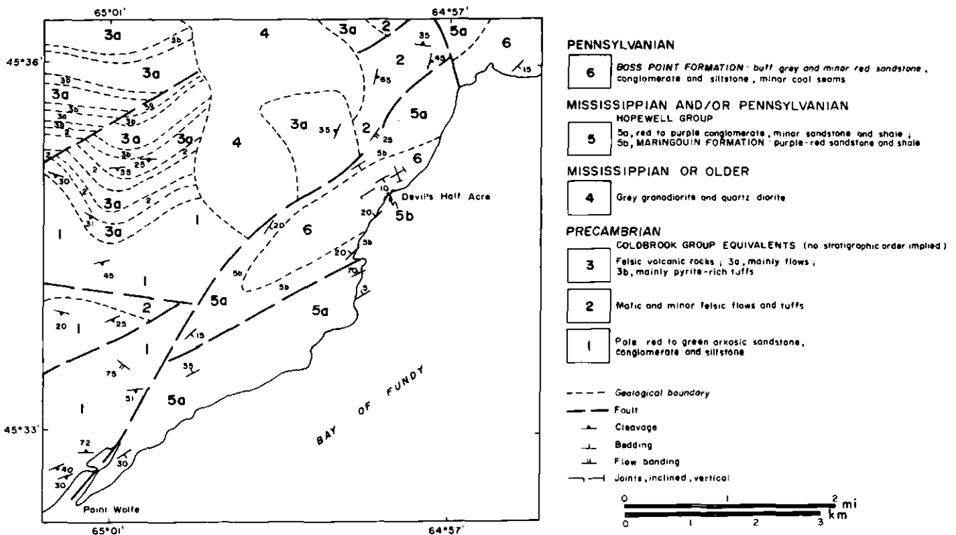
Figure 1 Geological sketch map, Devil's Half Acre area (modified after Kindle, 1958 and Ruitenber et al., 1975).
