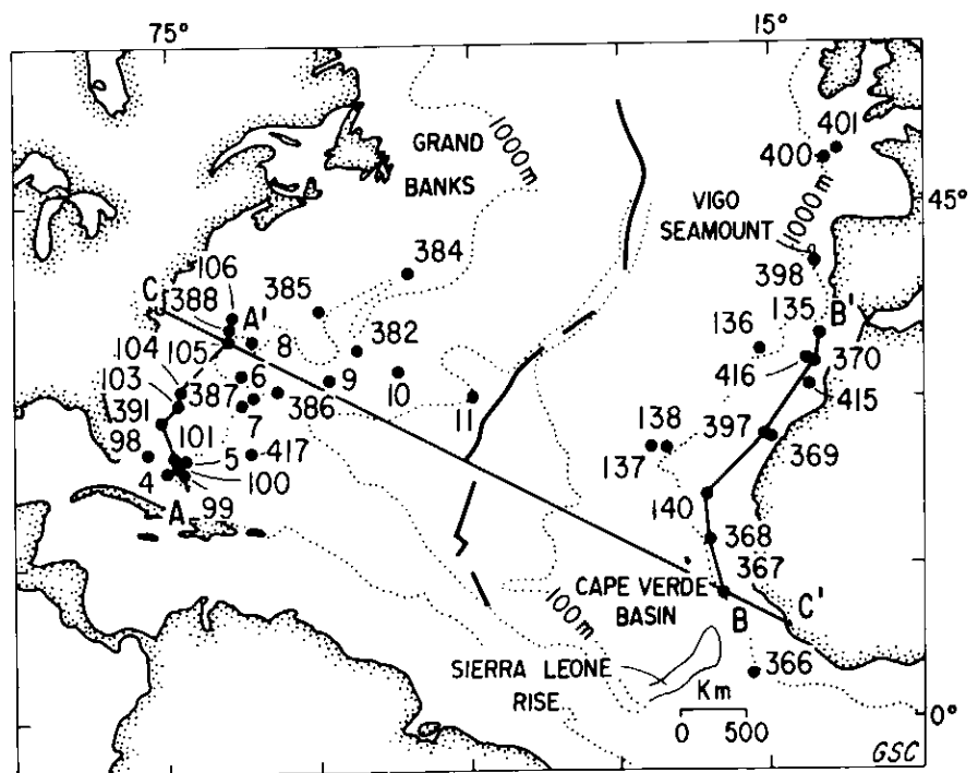
Figure 1 Location map, Central North Atlantic Basin. AA', BB', CC' are lines of cross-section shown on Figures 4, 5, and 6. Numbered
