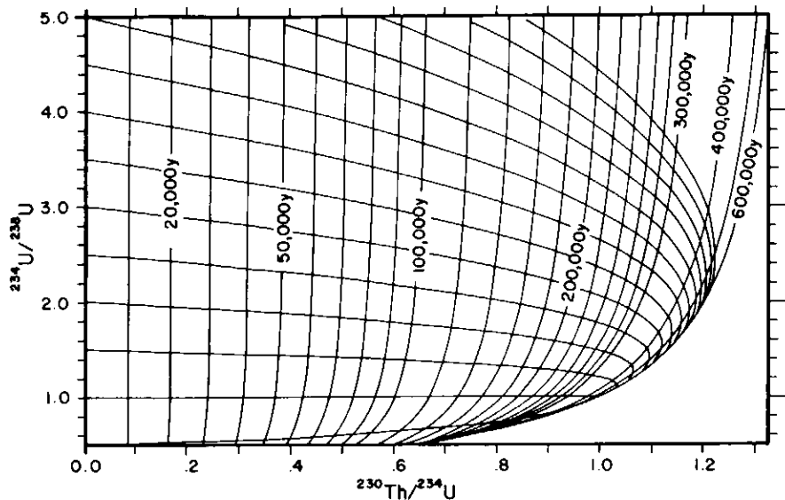
Figure 2 Relation between ^{234}\text{U}/^{238}\text{U} and ^{230}\text{Th}/^{234}\text{U} ratios for closed systems initially free of ^{230}\text{Th} . The subhorizontal curves are decay paths for samples initially deposited with ^{234}\text{U}/^{238}\text{U} ratios equal to left-hand ( ^{230}\text{Th}/^{234}\text{U}=0 ) intercepts. The steep curves are isochrons, in years.
