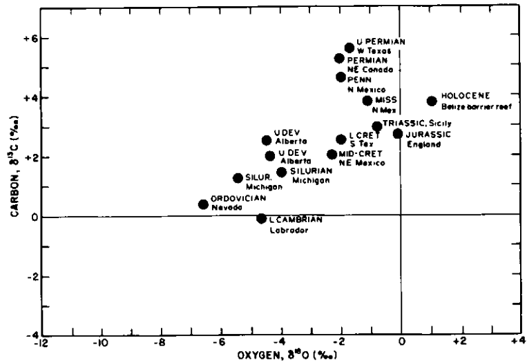
Figure 20 Crossplot of carbon versus oxygen isotopic compositions of Holocene and ancient fibrous and spherulitic (botryoidal) carbonate cements. The values shown are the "heaviest" compositions from covariate populations of data, believed to approximate most closely the original marine-isotopic compositions of the cements (method of Lohmann, in press). The data are from James and Ginsburg (1979),
