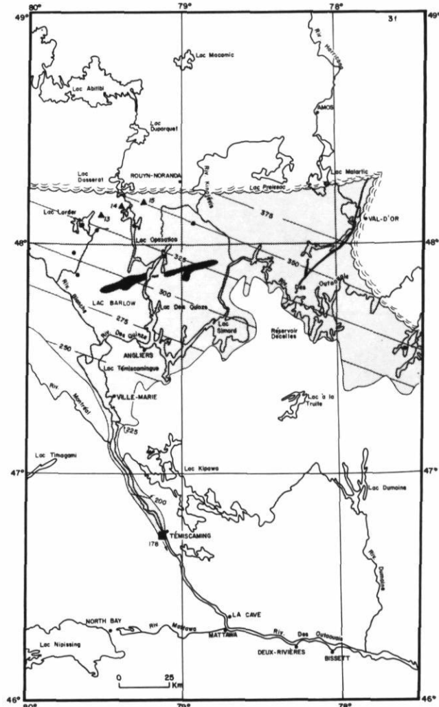
FIGURE 3f. Reconstitution schématique des phases lacustres: lac Barlow, phase de Témiscaming. Schematic reconstruction of the lacustrine phases: Lake Barlow, Temiscaming Phase.
