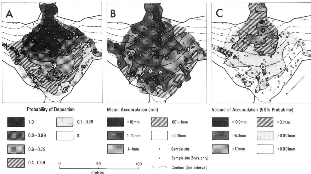
FIGURE 7. Depositional patterns on the Tumblin' Creek Cone (1968-1978). A: The probability of receiving deposition in any year; B: Mean annual accumulation on sample sites; C: Volume of accumulation equalled or exceeded one year in two (50% probability map). The isolines are drawn at 0.5 probability, e.g. the sites within the lightest stippled area received deposition of between 0.0001 and 0.1 mm for at least five of the ten years between 1969 and 1978 (see text). Note: in these diagrams volumes of accumulations are reported as depth (thickness) in millimetres.
