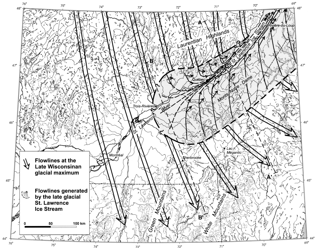
FIGURE 10. Reorientation of Late Wisconsin flowlines generated by the St. Lawrence Ice Stream. Lines A-A' and B-B' show the location of schematic cross-sections of Figures 11 and 12.
