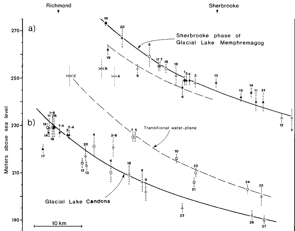
FIGURE 4. Shoreline diagram for the Sherbrooke Phase of Glacial Lake Memphremagog (a) and for Glacial Lake Candona (b). Line of section and location of shoreline features of Glacial Lake Memphremagog are given in Figure 3 with the same symbols. Lake Candona features follow the same numbering as in Parent and Occhietti (1988). Dashed vertical lines show the probable measurement error of elevation data.
