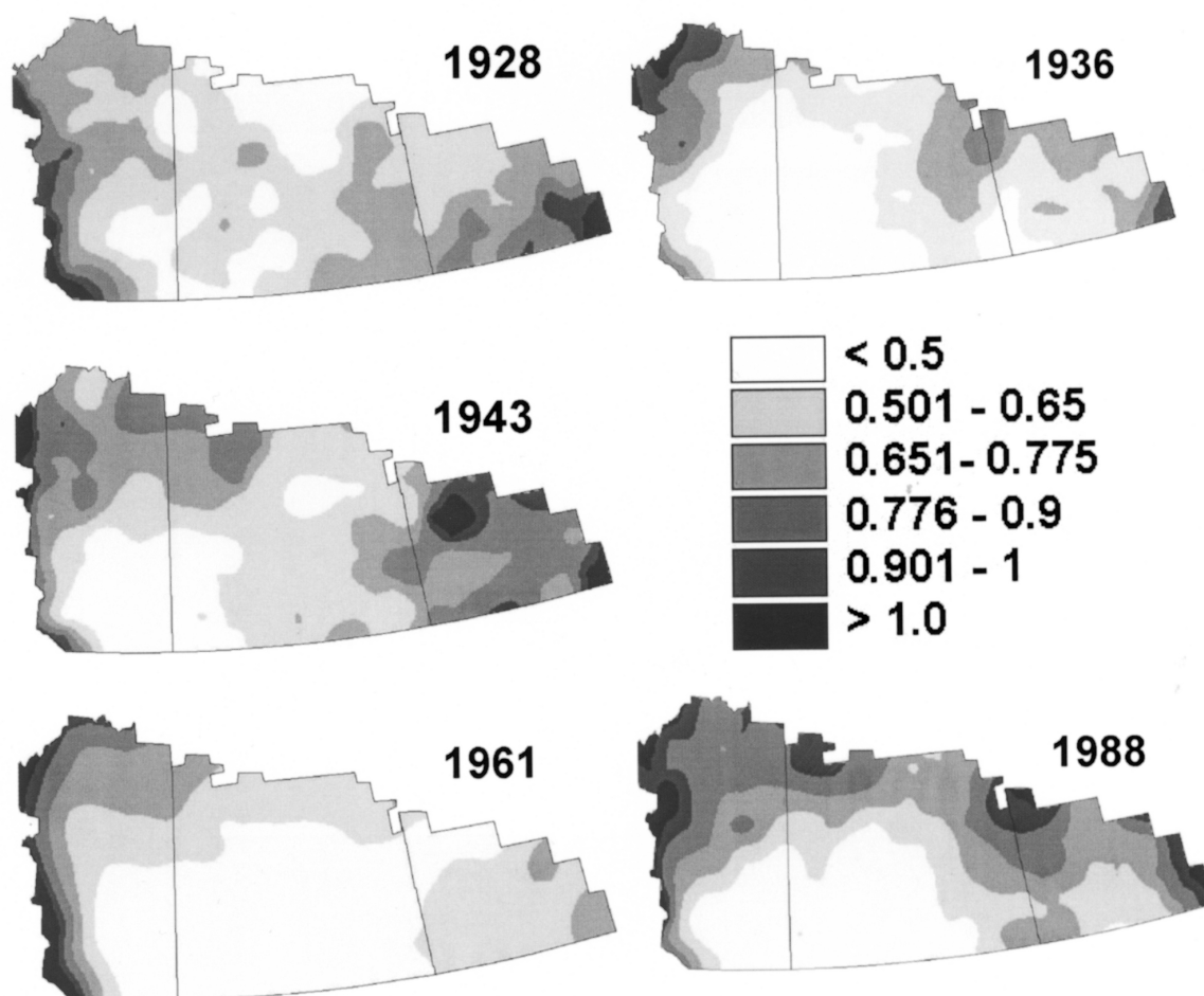
FIGURE 4. Annual aridity index for five drought years for the agricultural zone of the Prairie Provinces. During the drought years, aridity index was < 0.5 (semiarid) over a large part of the agricultural zone. The most extensive drought was in 1961.
