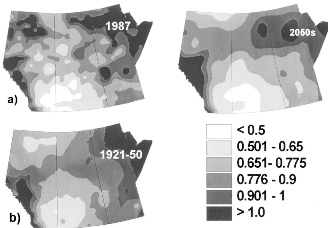
FIGURE 11. a) P/PET in 1987 and forecasted for the 2050s, showing that a dry year like 1987 can serve as an analogue of the extent of semiarid and dry subhumid climate expected by the 2050s under a warm and dry climate change scenario (CGCM2 A21). b) An aridity map for the Prairie Provinces for the period 1921-1950. In contrast to the "normal" climate for 1961-1990 (Fig. 2), the climate of 1921-1950 is drier throughout the Prairie Provinces and there are two small areas of semiarid climate ( P/PET < 0.5 ) along the Alberta-Saskatchewan boundary.
