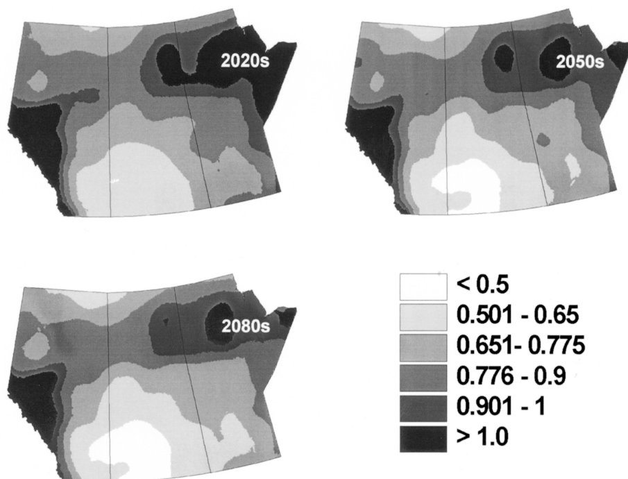
FIGURE 5. Aridity scenarios for the 2020s, 2050s and 2080s based on forecasts of precipitation and temperature from the Canadian GCM, CGCM2, the warm-dry climate change scenario. A small area of semi-arid climate ( P/PET < 0.5 ) appears in western Saskatchewan by the 2020s and then expands significantly by the 2050s with further increase in the area of semi-arid and subhumid climate by the 2080s.
