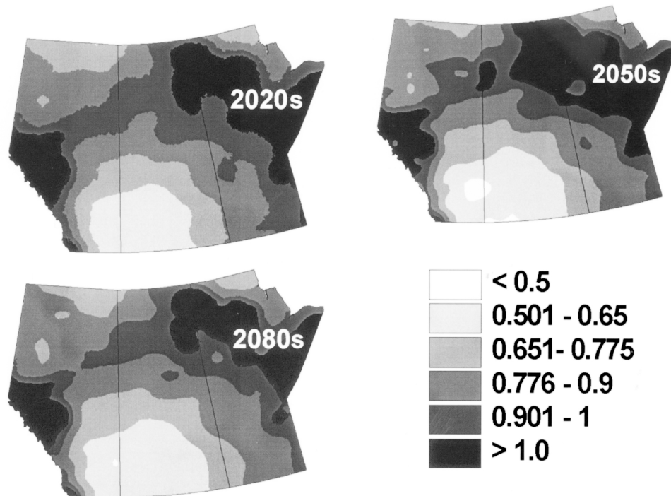
FIGURE 7. Aridity scenarios for the 2020s, 2050s and 2080s based on forecasts of precipitation and temperature from the UK Hadley Centre GCM, HadCM3, the cool-wet climate change scenario. This scenario forecasts the least change in climate. There is a marginal increase in the area of subhumid climate with maximum aridity occurring in mid-century.
