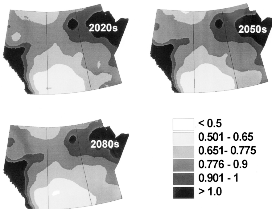
FIGURE 6. Aridity scenarios for the 2020s, 2050s and 2080s based on forecasts of precipitation and temperature from the Australian GCM, CSIRO Mk2b, the mid-range climate change scenario. By the 2080s, dry subhumid climate extends as far east as southwestern Manitoba and an area of semi-arid climate appears in western Saskatchewan.
