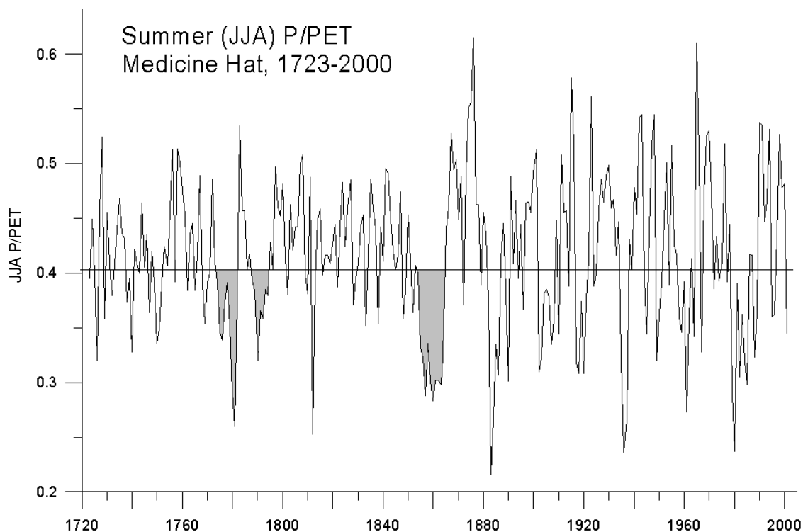
FIGURE 8. Proxy summer (JJA) aridity for Medicine Hat, Alberta as reconstructed from a residual index tree-ring chronology from Pinus contorta from the Cypress Hills. The gray fill highlights prolonged summer droughts of the 18 th and 19 th centuries. The straight line marks the mean aridity (0.415) for the period of record.
