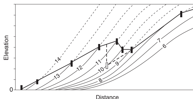
FIGURE 2. The schematic relationship between raised shoreline gradient, marine limit gradient, and rate of ice marginal recession. Numbered solid lines are the profiles of hypothetical raised shorelines with the numbers indicating age in thousands of years. Thick vertical bars represent ice margins. The open bar represents a stillstand or readvance of the ice margin. Dashed extensions of the shoreline profiles represent the increase in elevation of the glacier bed since the times indicated. The heavy line connecting ice marginal positions is the marine-limit surface.
