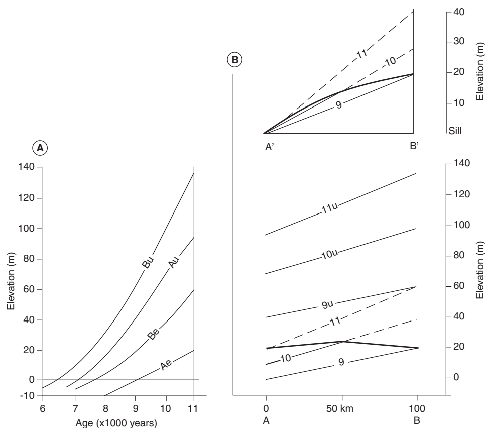
FIGURE 3. Relationship between a lake-limit surface and an adjacent marine-limit surface formed over the same time interval. (A) Emergence (Ae, Be) and uplift (Au, Bu) curves for sites A and B. (B) Site B is 100 km closer to the uplift centre than site A. Sites A and B are at marine limit. Site A' is at a glacial lake outlet sill on same isobase as site A. Site B' is on same isobase as site B. Numbered lines (9, 10, 11) are shoreline profiles; lines labelled 9u etc. show uplift profiles. Heavy lines represent marine-limit (lower) and lake-limit profiles (upper).
