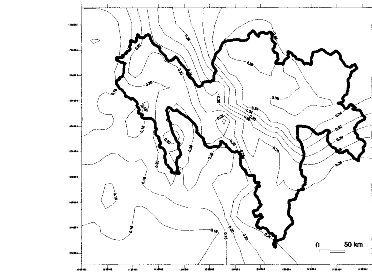
Figure 5 Coefficient de variation interannuelle des précipitations. Coefficient of variation of annual rainfall.
