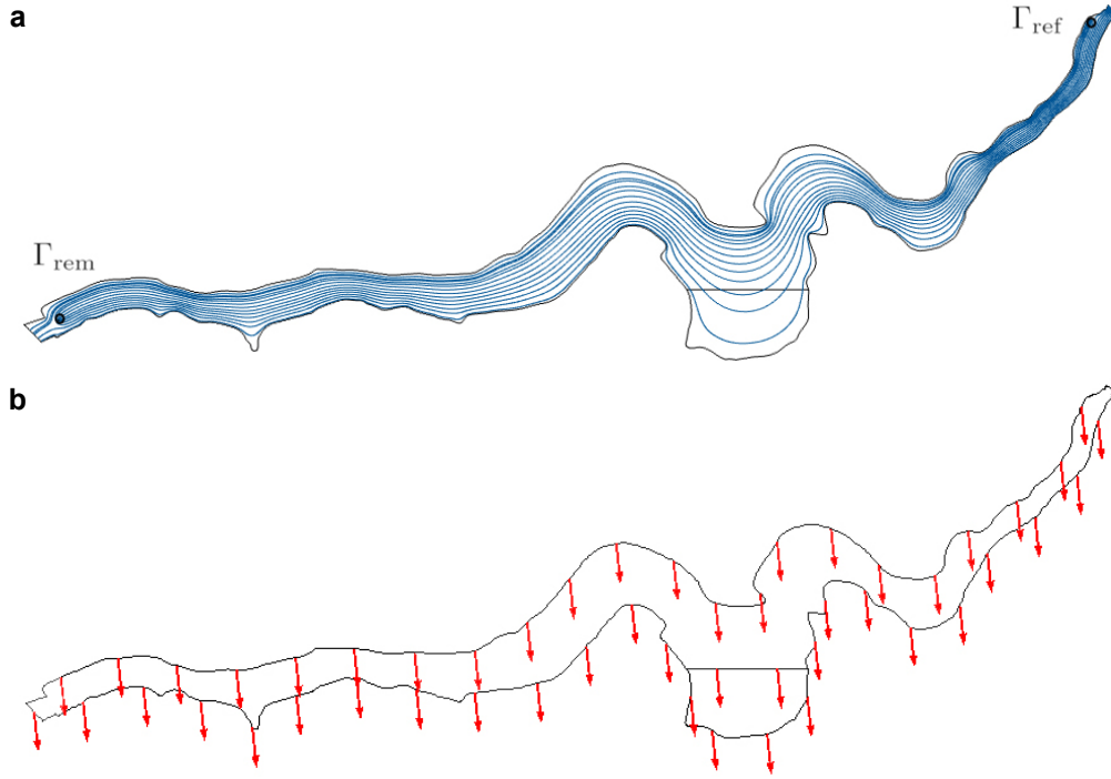
Figure 3. Analysis of the wind and water current velocity vectors for Jaunay Lake: a) water current streamlines associated to an specific choice of \Gamma_{ref} and \Gamma_{rem} , b) usual wind directions registered in the lake region.
