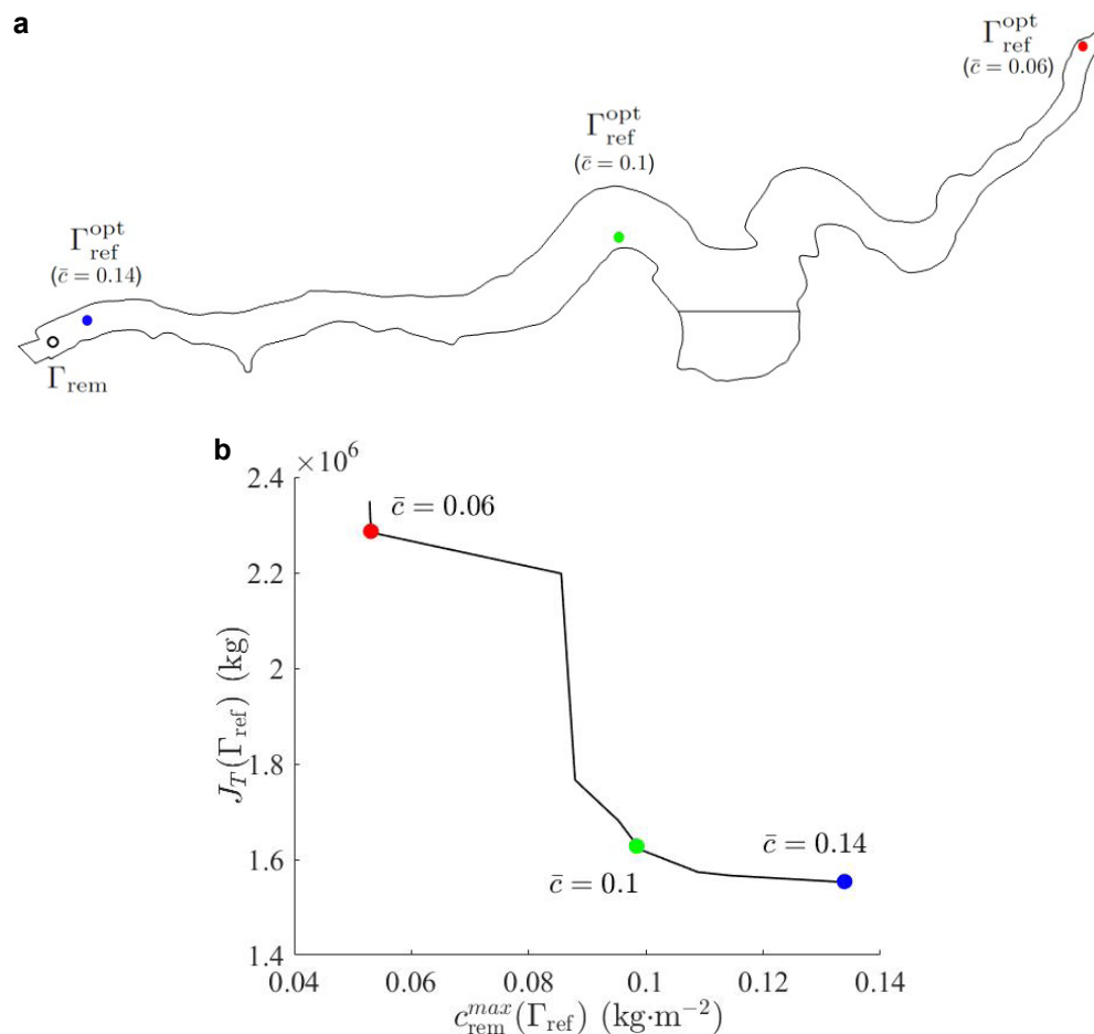
Figure 5. Graphical interpretation of the optimization results solution of equation 2 when \bar{c} \in \{0.06, 0.1, 0.14\} \text{ kg}\cdot\text{m}^{-2} : a) optimal refilling locations \Gamma_{ref}^{opt} , b) objective values J_T(\Gamma_{ref}^{opt}), c_{rem}^{max}(\Gamma_{ref}^{opt}) associated to these optimal refilling locations. The black curve represents the Pareto front.
