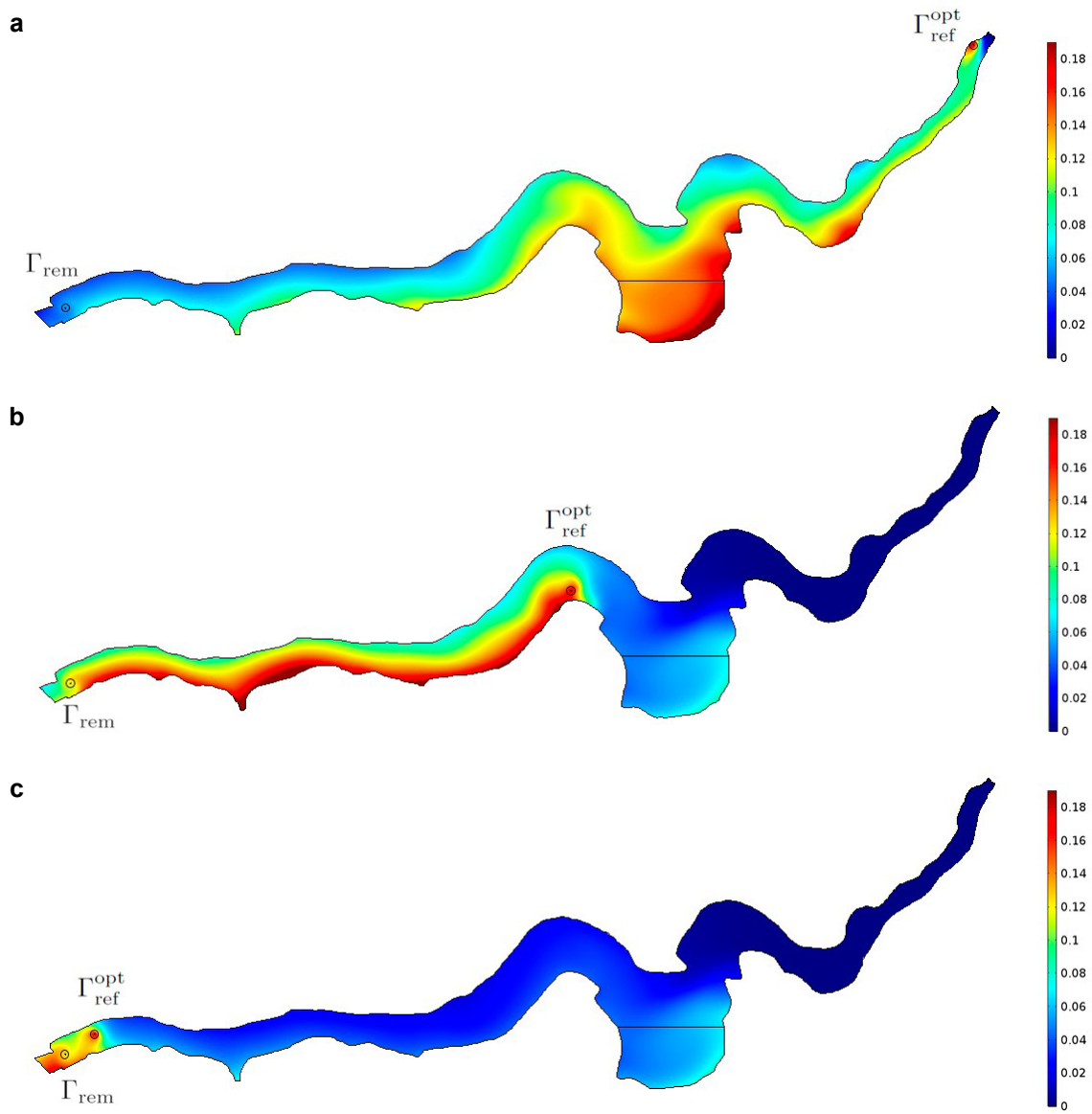
Figure 6. Pollutant concentration c ( \text{kg}\cdot\text{m}^{-2} ) at the simulated final time (31 August 2016) associated to the optimal refilling locations \Gamma_{\text{ref}}^{\text{opt}} solution of equation 2 when \bar{c} = a) 0.06, b) 0.1, c) 0.14 \text{kg}\cdot\text{m}^{-2} .
