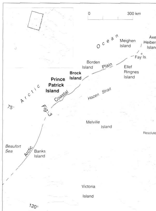
FIGURE 1. Location of western Canadian Arctic Archipelago, Arctic Coastal Plain and study area.
