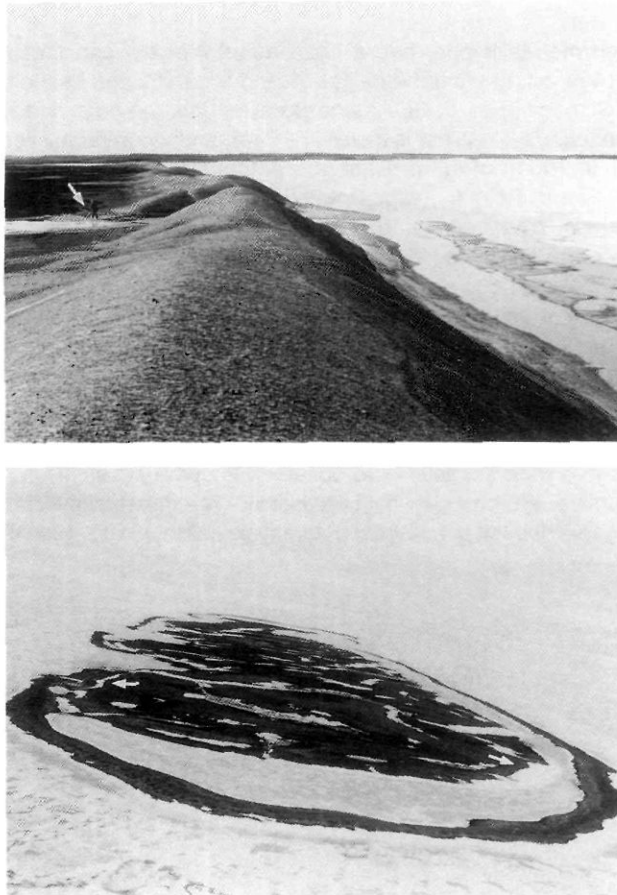
FIGURE 7. a) Ground view of the sea ice-built ridge at the present shoreline on west-central Prince Patrick Island (person indicated by arrow). b) Aerial view (July, 1990) of the sand and gravel ridge that encircles the southern of the two Polynia Islands, Ballantyne Strait. The island is 1 km wide. The ridge at the present shoreline is 30-50 m wide, and extends to 4 m asl. A second less continuous ridge lies at 5-8 m asl (arrows).
