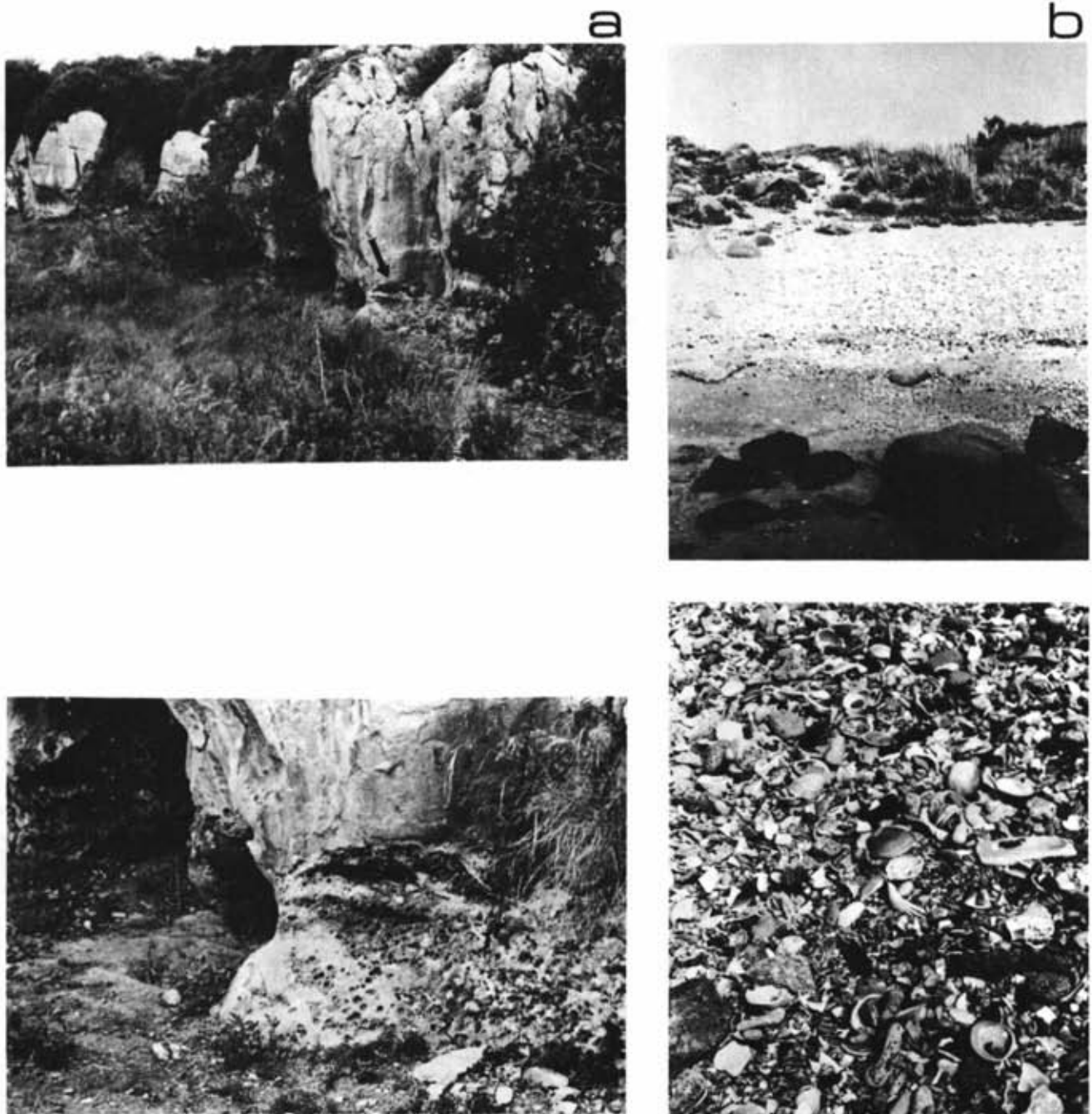
FIGURE 4. Recent indicators of Holocene transgression on the Mediterranean coast. A) Calcareous cliff (Mesozoic) of Cap Romarin showing a littoral facies and holes caused by shells and molluscs due to a positive level (+2m) of the Holocene sea. At the foot of the cliff (detailed photo) the sandbar dated 4100 to 4500 years BP resulting from sedimentary infilling of the plain. B) Shell accumulations on Rochelongue Beach (Cap d'Agde). The upper photo offers a general view of the formation and basaltic blocks outflow of the Quaternary volcano of Agde on the shore. Lower photo shows the abundance and variety of the shells mixed with pebbles and sands different in nature and origin. Dates on this material range from the Present to 4700 y BP.
