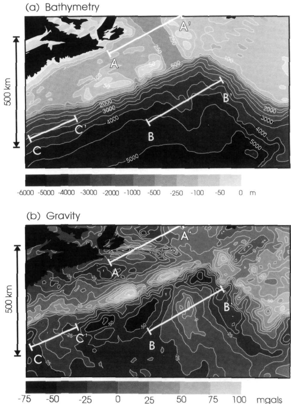
FIGURE 2. a) Bathymetry in metres calculated from the Atlantic Geoscience Centre database. Contour lines are drawn at every transition and midpoint in the grey scale bar. b) Observed free-air gravity anomaly on the Scotian margin deduced from ship measurements. Contour lines are drawn at 12.5 mgal intervals.
