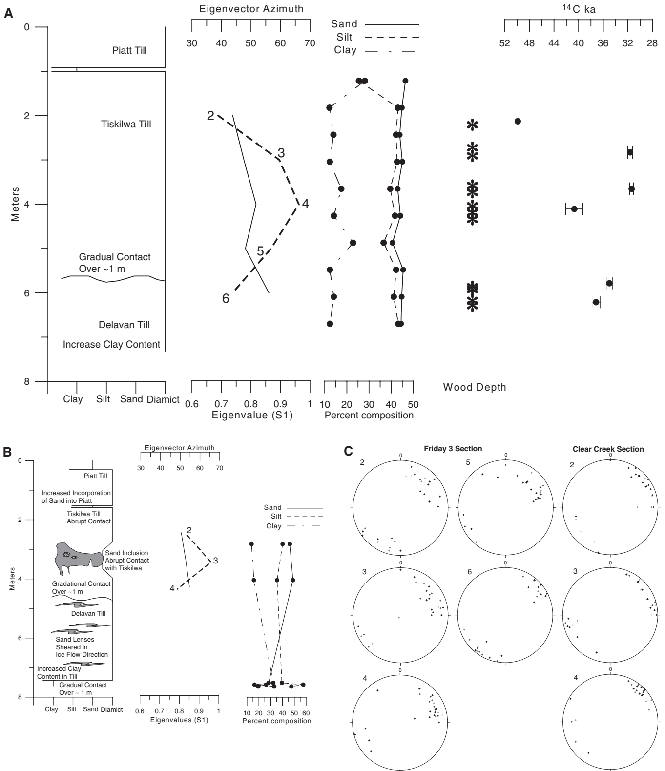
FIGURE 4. Tiskilwa Till section data. (A) Friday 3. (B) Clear Creek. Solid line is eigenvalues and dashed line is eigenvector azimuth. The radiocarbon date at 2.1 m from Friday 3 is >49.9 ^{14}\text{C} ka BP. (C) Pebble orientation from Friday 3 and Clear Creek. Numbers indicate the depth (m) in the section from which the data were collected.
