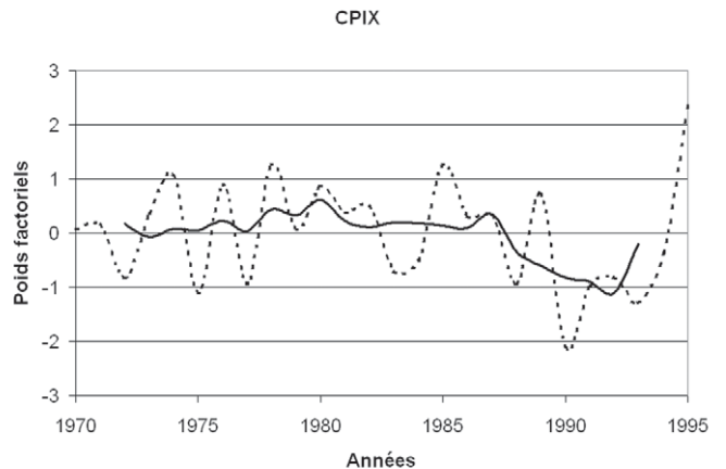
Annual variability of loadings for the principal components included in the fifth mode. The bold line represents smoothed values.
