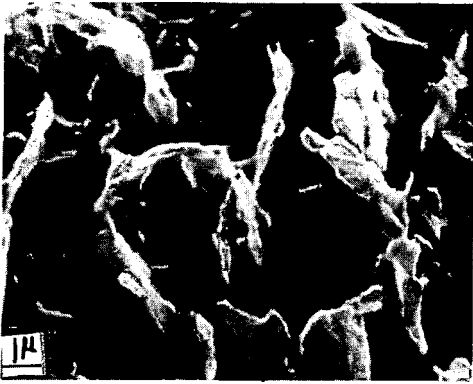
Figure 1 - Scanning electron micrograph of freeze-dried grundite illite floccules. Flocculated in distilled water. x 8000.
