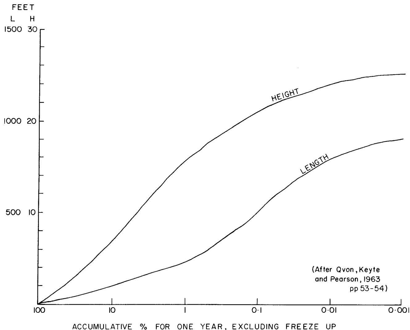
Figure 1 - Probability of occurrence of waves of particular lengths and heights in southern Gulf of St. Lawrence.
