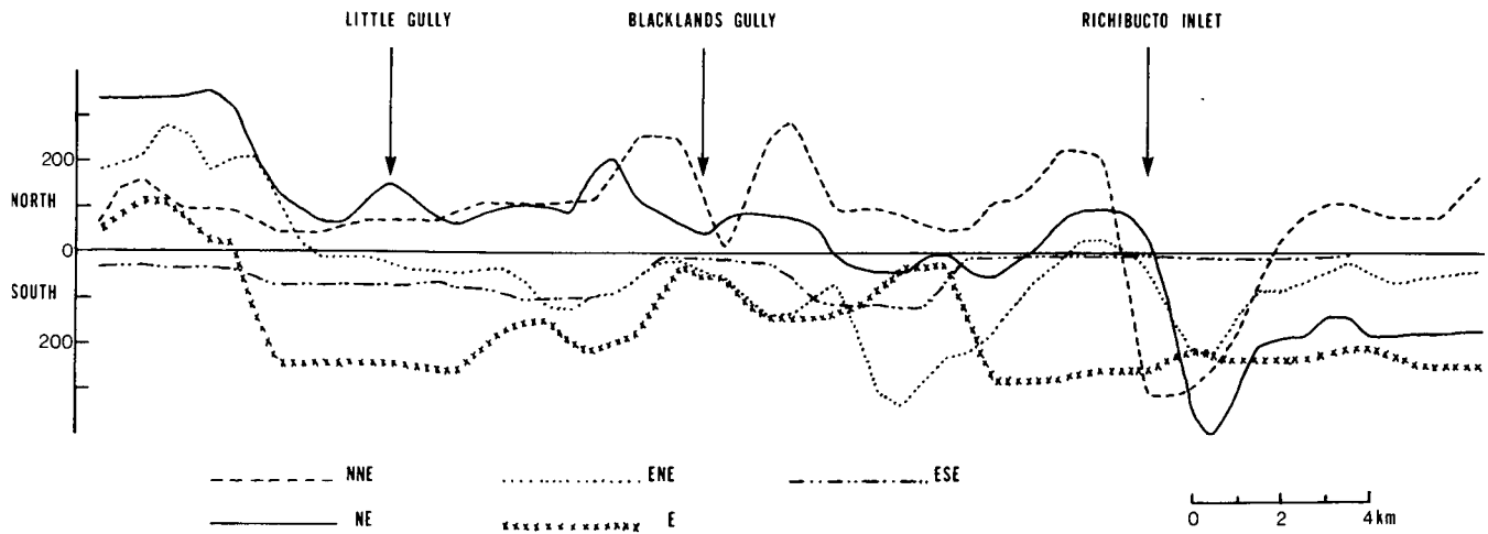
FIG. 5 Variation in the directional residual component of longshore wave power for NNE-ESE wave directions between Richibucto Head and Lower Sapin (gm cal/m/sec).
