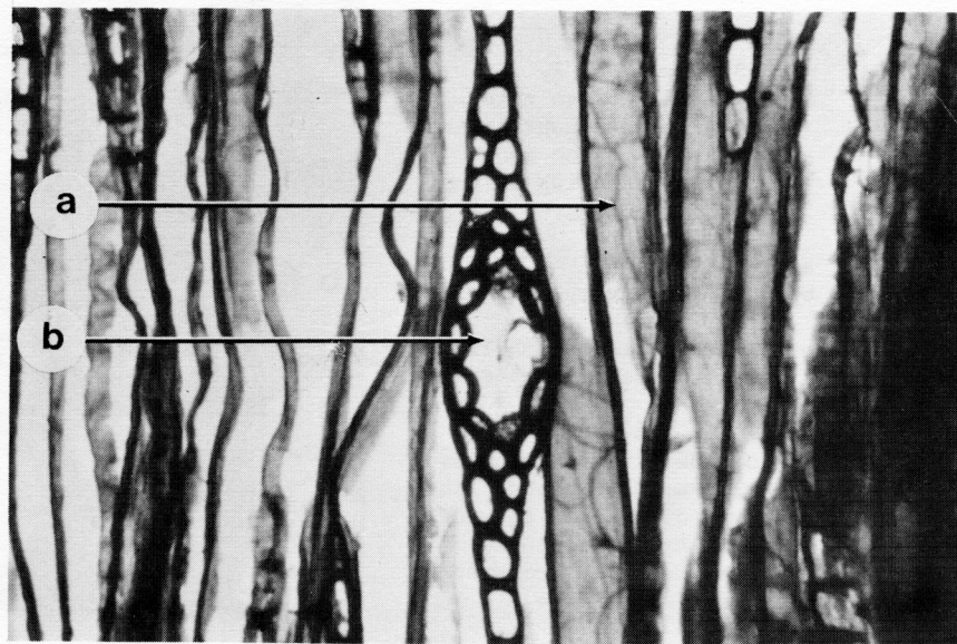
Fig. 1. Wood Specimen No. 2. Tangential section of wood showing horizontal resin ducts and partially collapsed tracheids, some with fungus strands. (320X)
