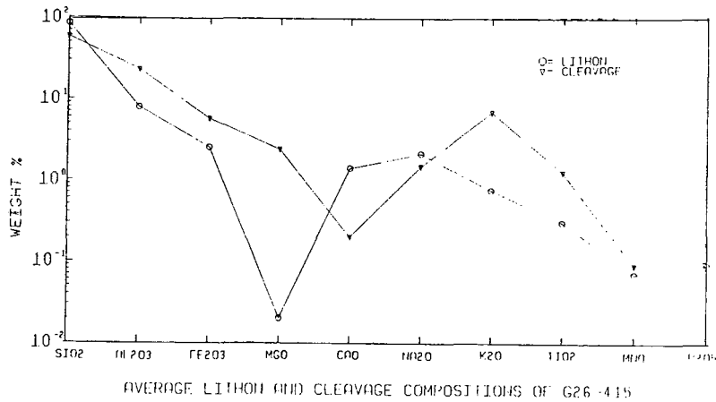
Figure 9 - Composition of the chemistry of lithons and CZ in sample # G26 - 415.
