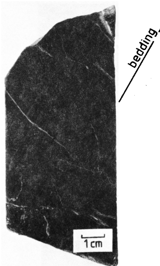
Figure 15 - Core sample of conformable galena and sphalerite (grey) in black slate. Small cross-cutting veinlets contain sphalerite. The section that includes this sample assayed 2.24 % Pb and 5.36 % Zn.
