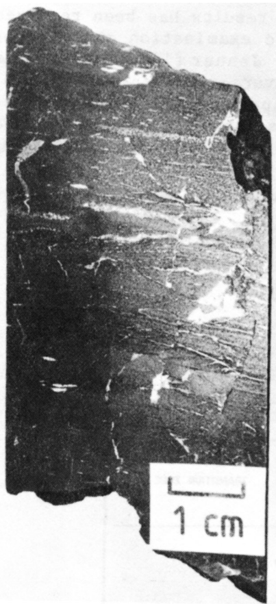
Figure 17 - Discontinuous spherulitic and galena veinlets and adjacent disseminations in black slate.
