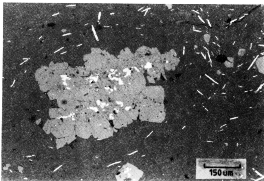
Figure 14 - Calcareous quartzite member containing small rutile needles with a preferred orientation around a porphyroblast of garnet (grey) enclosing minor sphalerite (white) (reflected light).
