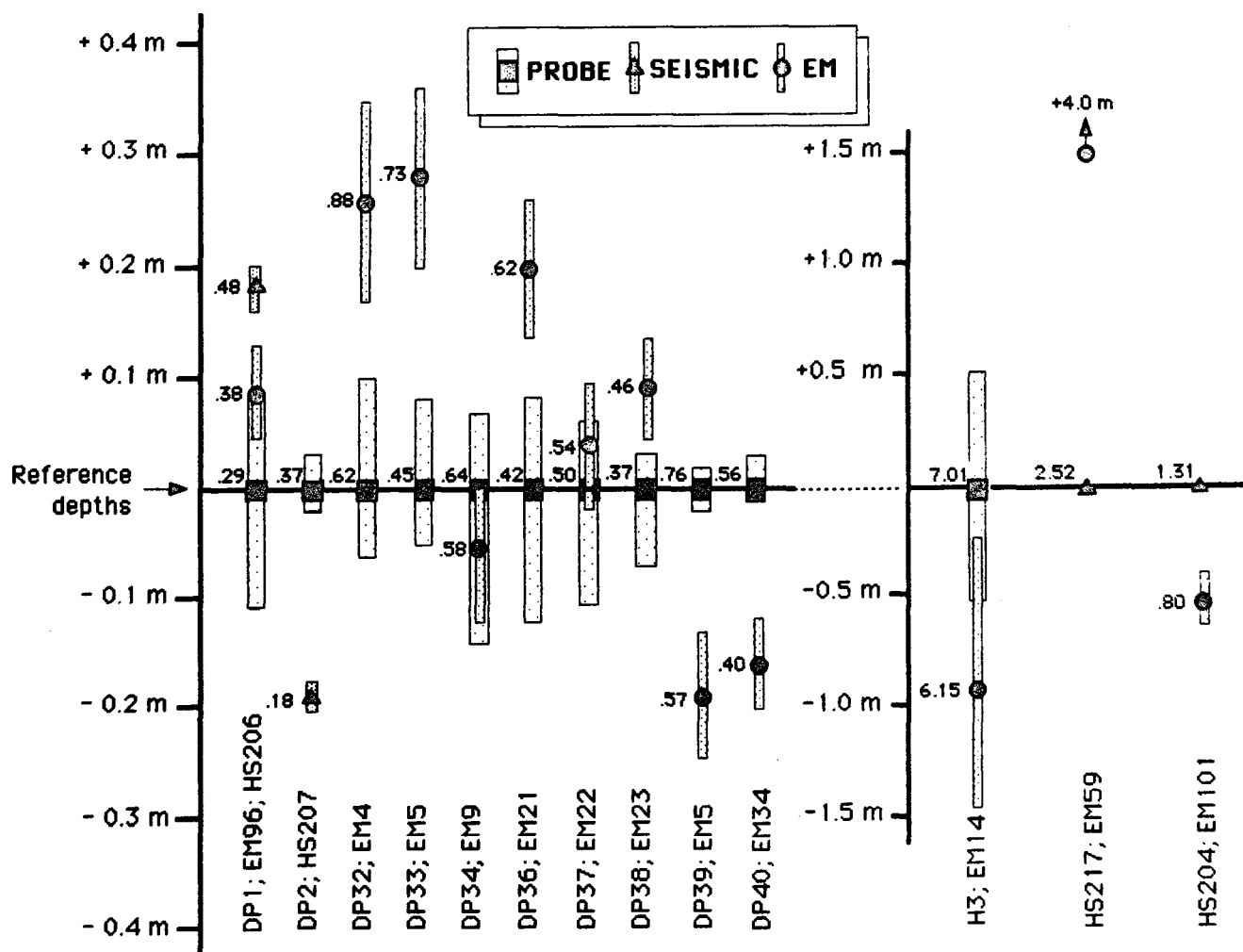
Fig. 4. Comparative results of depth to bedrock for ground truth and geophysical methods (see text for discussion).
