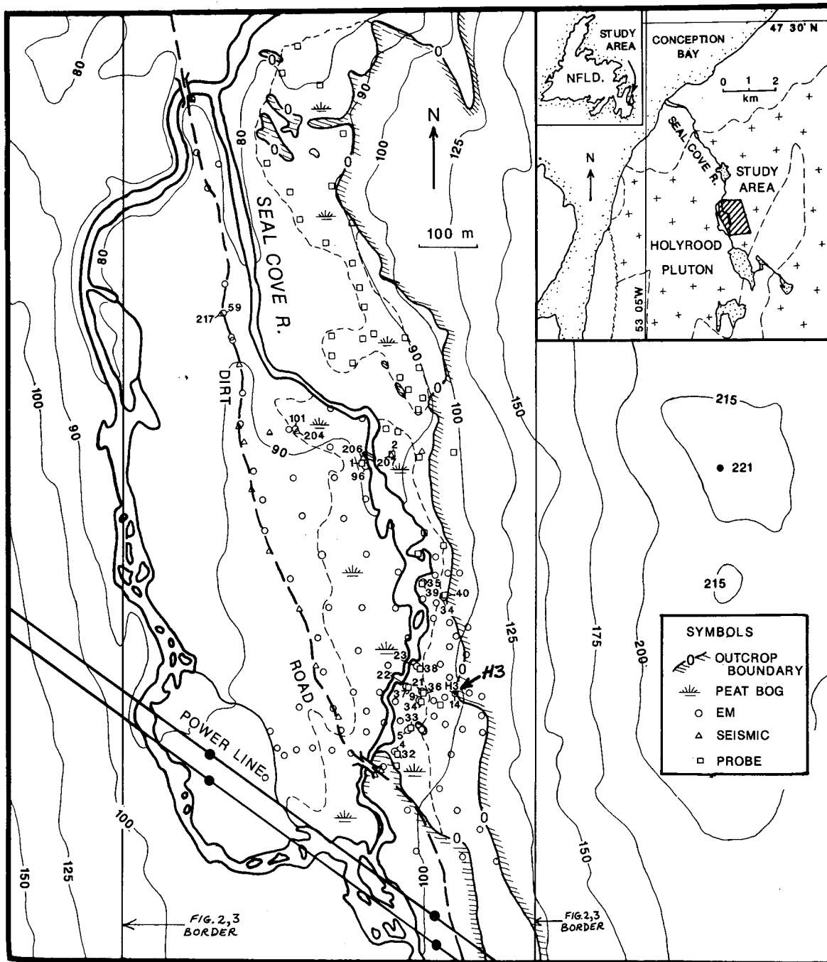
Fig. 1. The Seal Cove River valley showing topography, survey locations, bog areas and outcrop boundaries ("0" contour line); the vertical lines within the map show the borders for Figs. 2 and 3; the insets show location and geological setting of the study area; all contours in meters; north is true north for this and all other Figures.
