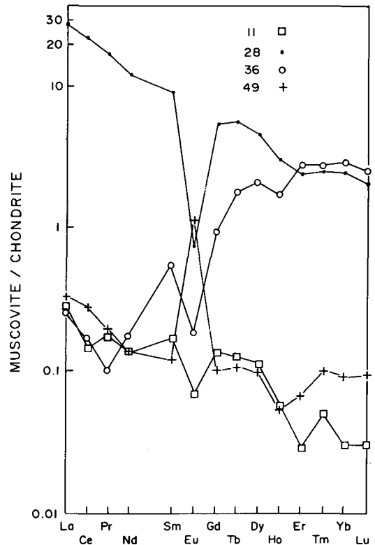
Fig. 2. Chondrite-normalized REE profiles for muscovite samples, South Mountain Batholith.
