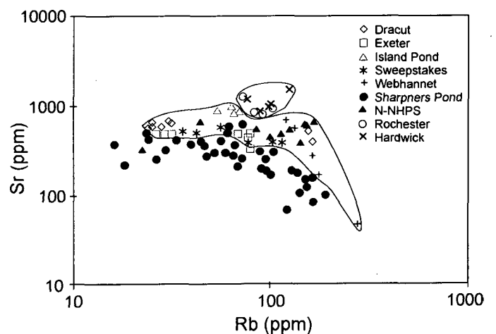
Fig. 14. Sr vs. Rb diagram for the Merrimack belt, the New Hampshire Plutonic Suite (N-NHPS), the Sharpners Pond, Rochester, and Hardwick plutons. The New Hampshire Plutonic Suite and Merrimack belt plutons are identical in composition. The Sharpners Pond samples are poorer in Sr at equivalent values of Rb compared to those of the Merrimack belt and New Hampshire Plutonic Suite. The Rochester and Hardwick samples are again identical in composition, plotting at higher Sr values than the other samples.
