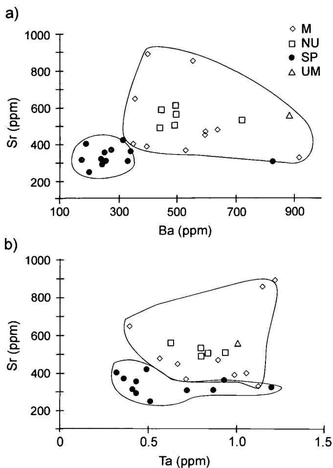
Fig. 15. a) Sr vs. Ba and b) Sr vs. Ta diagrams for samples from the Merrimack belt (M), Nulhegan (NU), Umbagog (UM), and Sharpers Pond (SP) plutons. The Merrimack belt and New Hampshire Plutonic Suite samples (NU and UM) plot within the same fields. In contrast, the Sharpers Pond samples are distinct from those of the Merrimack belt and New Hampshire Plutonic Suite.
