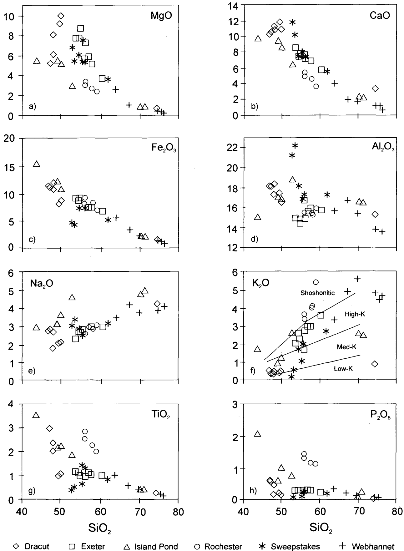
Fig. 8. Harker diagrams plotting major and minor elements versus \text{SiO}_2 . \text{K}_2\text{O} versus \text{SiO}_2 classification fields (f) after Gill (1981).
