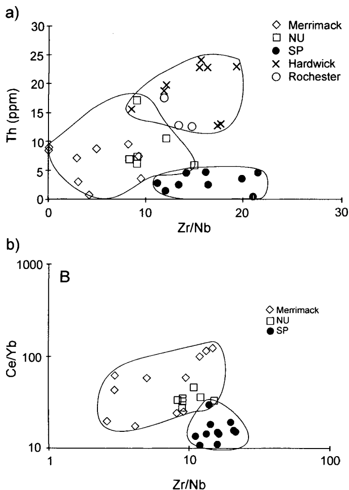
Fig. 16 a). Th versus Zr/Nb diagram for Merrimack belt, Nulhegan (NU), Sharpers Pond (SP), Rochester, and Hardwick plutons. The Merrimack belt and the Nulhegan pluton of the New Hampshire Plutonic Suite plot in the same field. The Rochester and Hardwick plutons are likewise identical whereas the Sharpers Pond samples plot in a distinct field. b). Ce/Yb versus Zr/Nb diagram showing that the Merrimack belt and the Nulhegan pluton of the New Hampshire Plutonic Suite plot in the same field. As above, the Sharpers Pond samples plot in a field that is distinct from the other samples.
