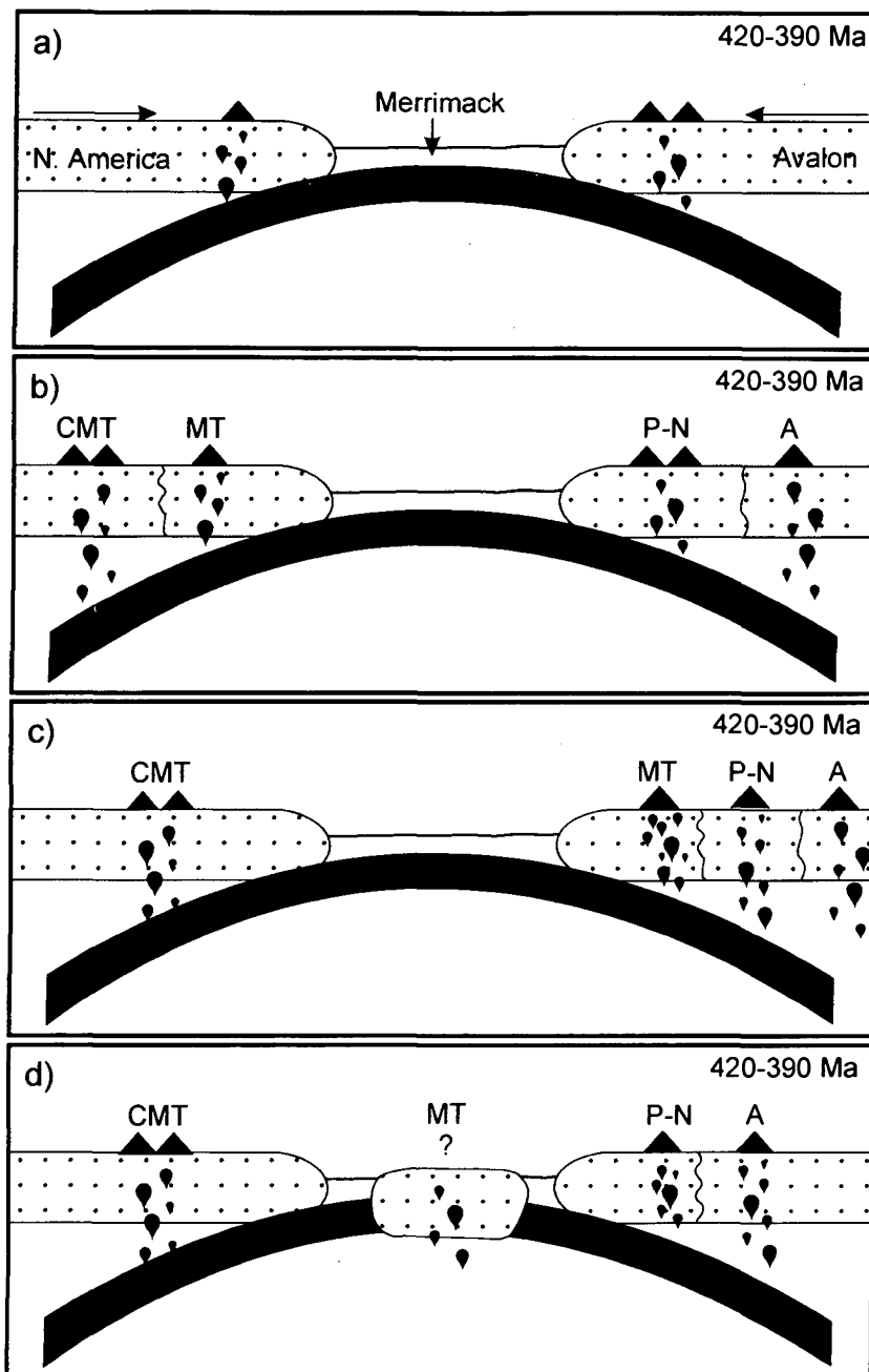
Fig. 3. Schematic diagram showing potential models for Late Silurian - Early Devonian magmatism in the Central Maine terrane, Merrimack belt, Putnum-Nashoba terrane, and the Avalon terrane. a) Molloy Sea type collision as visualized by various workers; b-d) Potential tectonic models (see text for discussion). CMT = Central Maine terrane; MT = Merrimack belt; P-N = Putnum-Nashoba terrane; A = Avalon Composite terrane.
