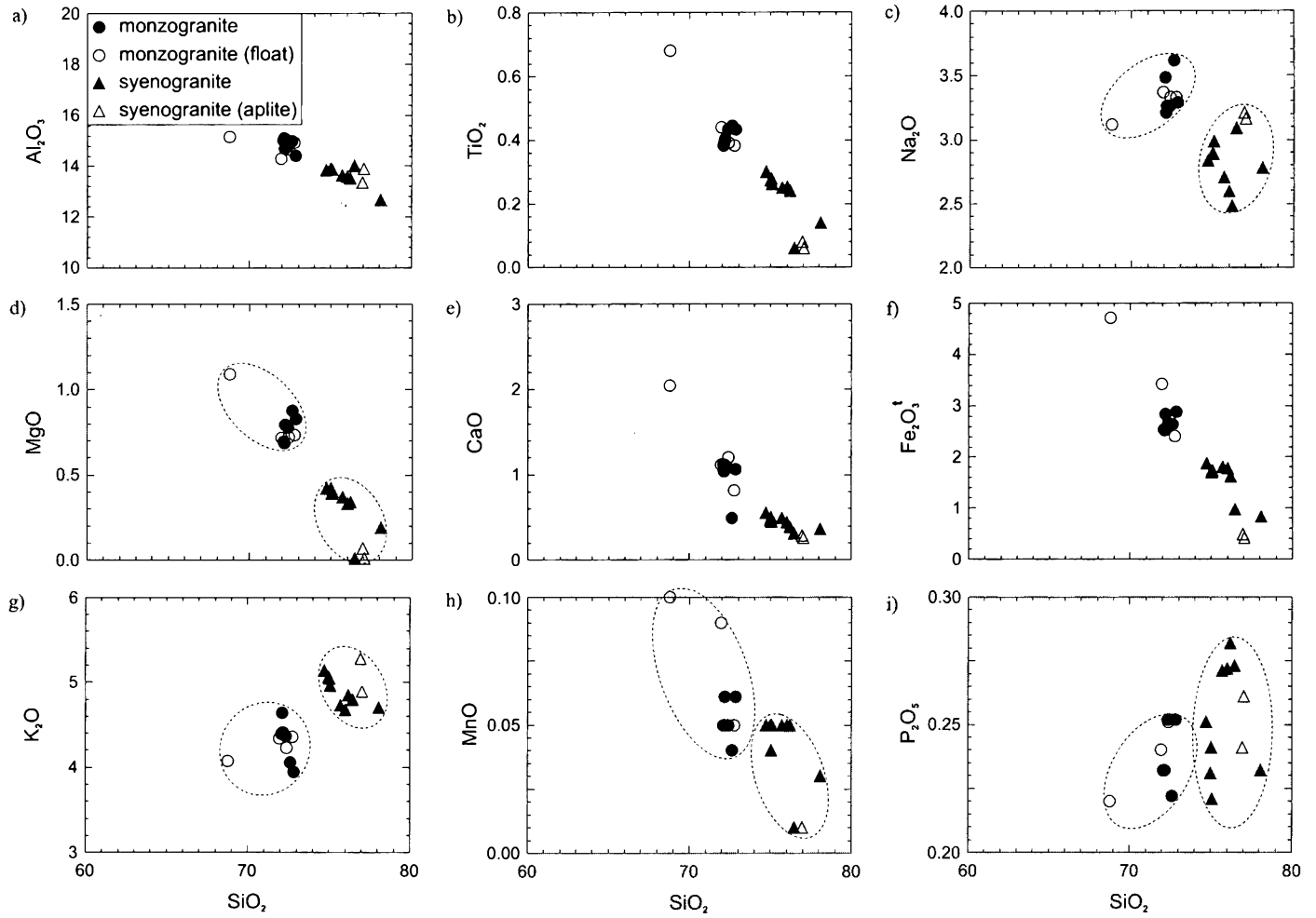
Fig. 7. Selected major elements plotted against SiO 2 (wt. %). Dashed lines outline clusters of monzogranite and syenogranite.
