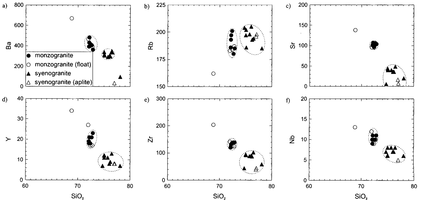
Fig. 8. Selected trace elements (ppm) plotted against SiO 2 (wt. %). Dashed lines outline clusters of monzogranite and syenogranite.
