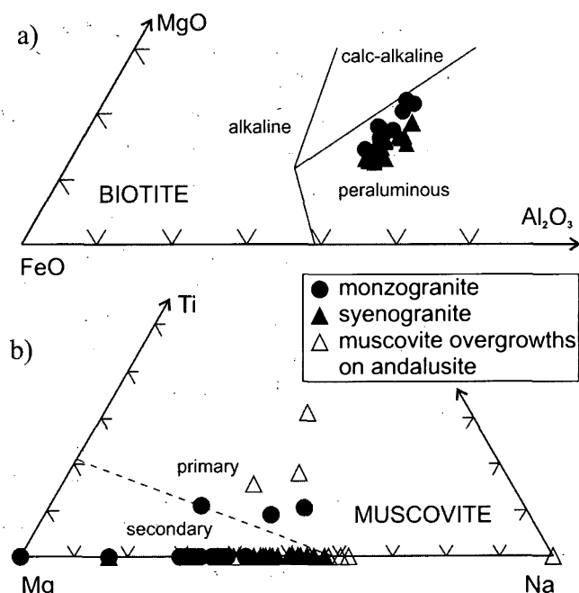
Fig. 16. Plots illustrating chemical variation in micas. a) Ternary variation for MgO, FeO, and Al 2 O 3 in biotite. Alkaline (A), calc-alkaline (C), and peraluminous (P) fields are from Abdel-Rahman (1994). b) Ternary variation for Ti, Mg, and Na in muscovite, with primary and secondary fields after Miller et al. (1981)
