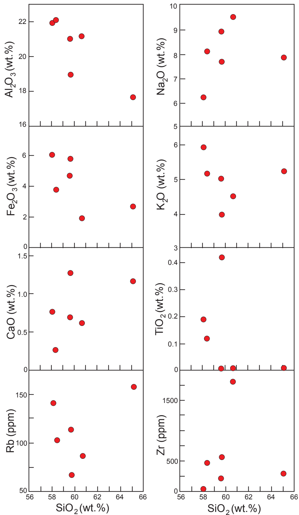
Figure 7. Harker geochemical variation diagrams illustrating the variability in \text{SiO}_2 and selected major (wt.% oxide) and trace (ppm) elements from representative rock types of the Litchfield pluton.
