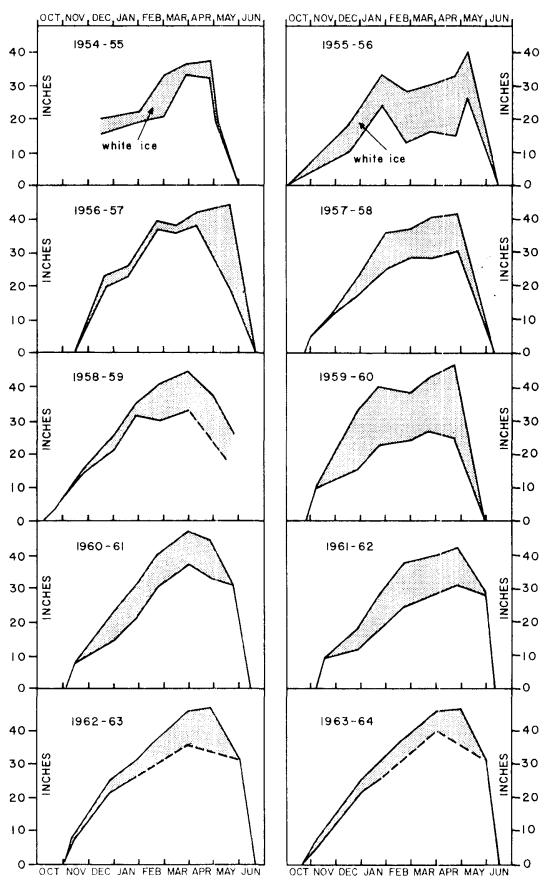
Figure 6 Annual growth of Knob Lake ice cover 1954-55 to 1963-64.
