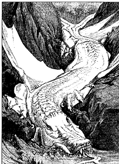
Figure 1 Dragon-glacier
