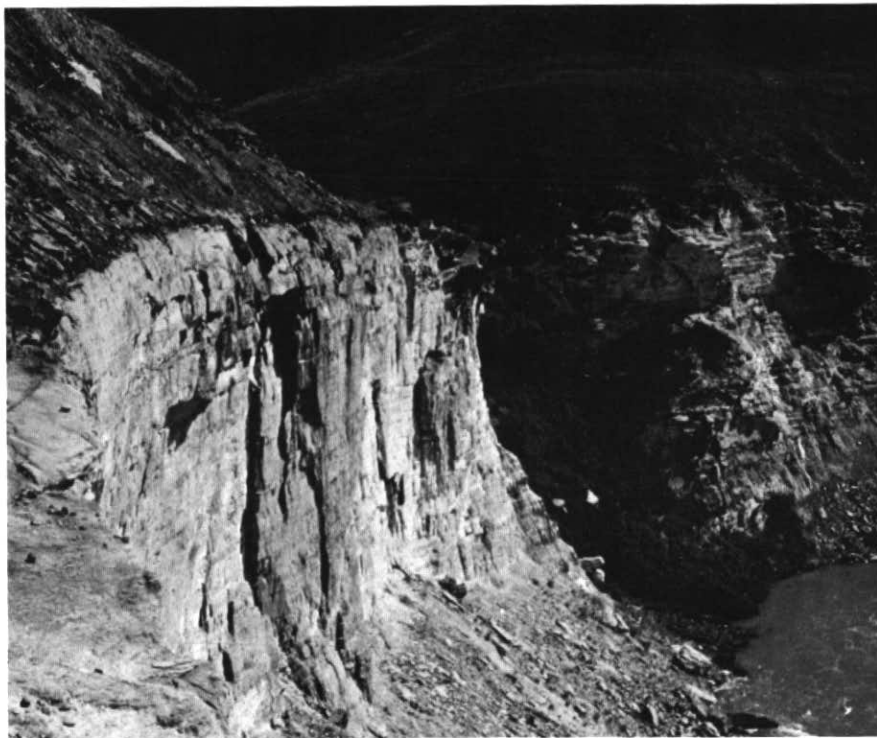
Figure 19 Photo showing the sharp contact between the clean sandstones of the Blood Reserve Formation and the overlying finer-grained lagoonal deposits of the St. Mary River Formation (vertical sequence illustrated in Fig. 16).
