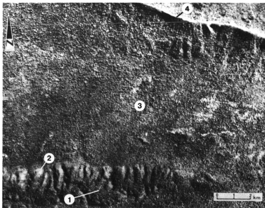
Figure 1 Aerial photograph showing nickel-laterite covered serpentinized peridotite (1),
