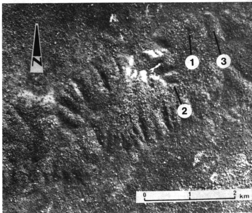
Figure 4 Aerial photograph of nickel-laterite covered serpentinized peridotite (same body as Figure 3).
