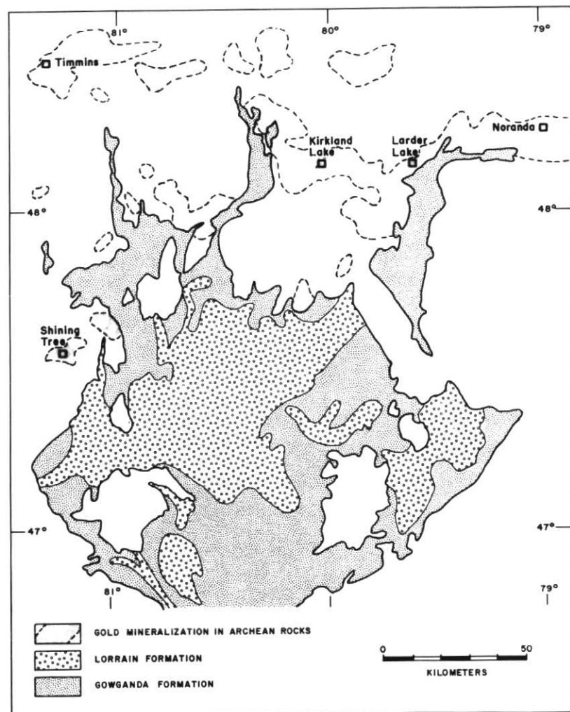
Figure 3 Generalized geology of the Cobalt Embayment and location of gold occurrences in basement rocks
