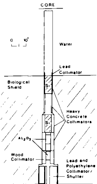
Figure 1 Cross section of the beam-port used to extract neutrons from the reactor core. Neutrons move from top to bottom in the diagram. They are filtered and thermalized by crystals of silicon (Si) and alumina ( \text{Al}_2\text{O}_3 ) and collimated by concrete, wood, lead and polyethylene. The final collimator may be rotated to shut off the neutron beam
