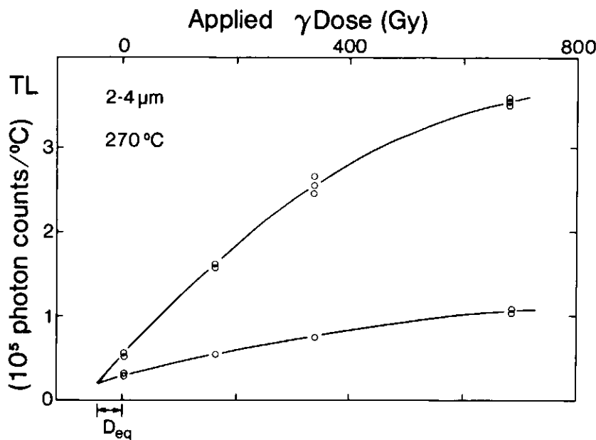
Figure 5 The measurement of equivalent dose ( D_{eq} ) by the partial bleach technique for the 2-4 \mu\text{m} polymineralic grains (feldspar dominated) from a thin winter varve of a glaciolacustrine deposit. From the plateau of D_{eq} values for the glow-curve temperature interval 260-320°C, a TL apparent age of 14 \pm 2 ka was calculated (after Berger, 1985c).
