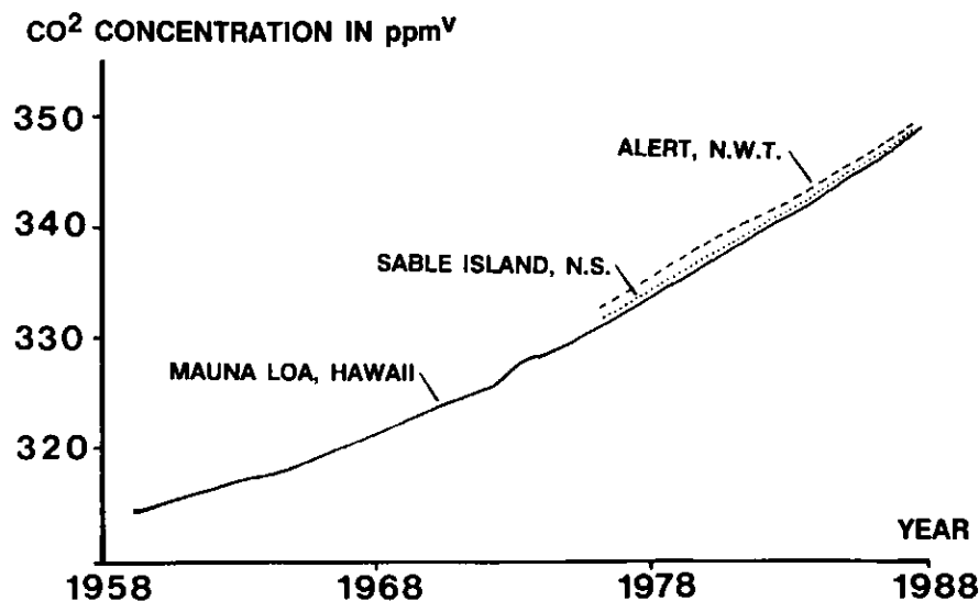
Figure 1 Increasing atmospheric concentrations of \text{CO}_2 measured over the last 30 years are illustrated in curves for Hawaii (Mauna Loa Observatory), and, more recently, for Canadian stations on Sable Island and at Alert. (Source: The Changing Atmosphere, Environment Canada).
