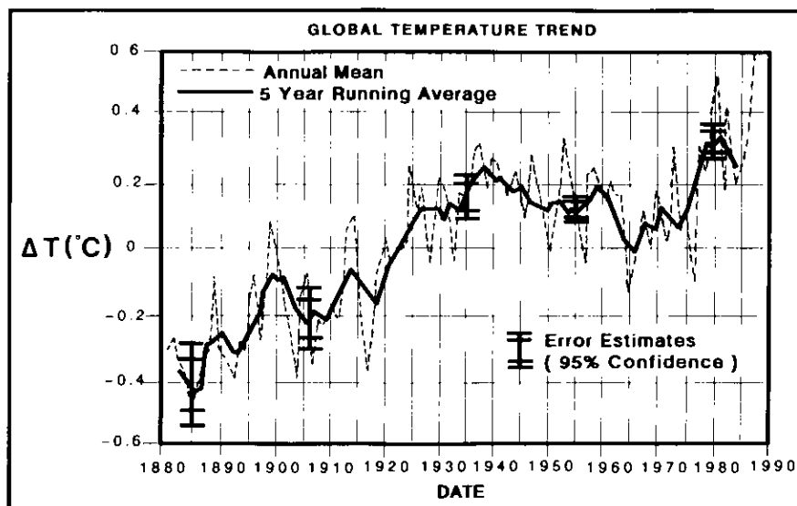
Figure 2 Global temperature trends have shown increasing values over the last century. Temperatures recorded during the decade of the 1980s are the highest observed with 1987 as one of the warmest on record. (Source: The Changing Atmosphere, Environment Canada).
