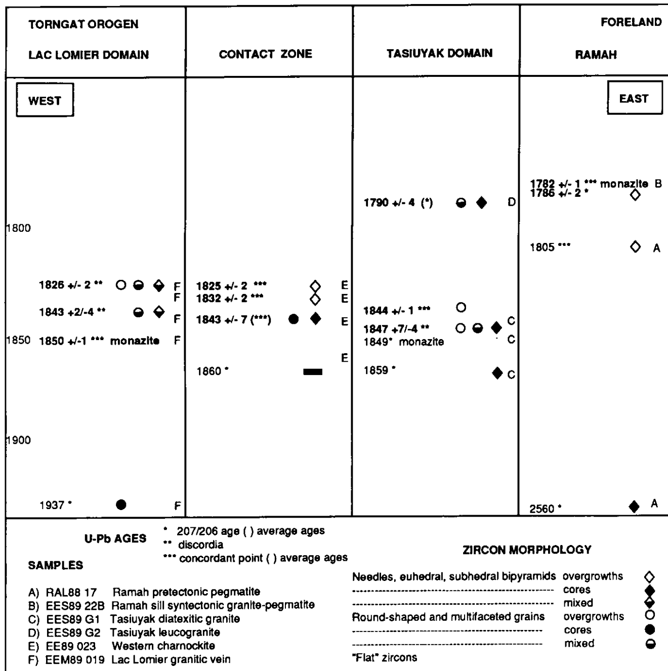
Figure 3 Time and space chart showing isotopic results and morphology of the analyzed samples. All ages are given with a 2\sigma error.
