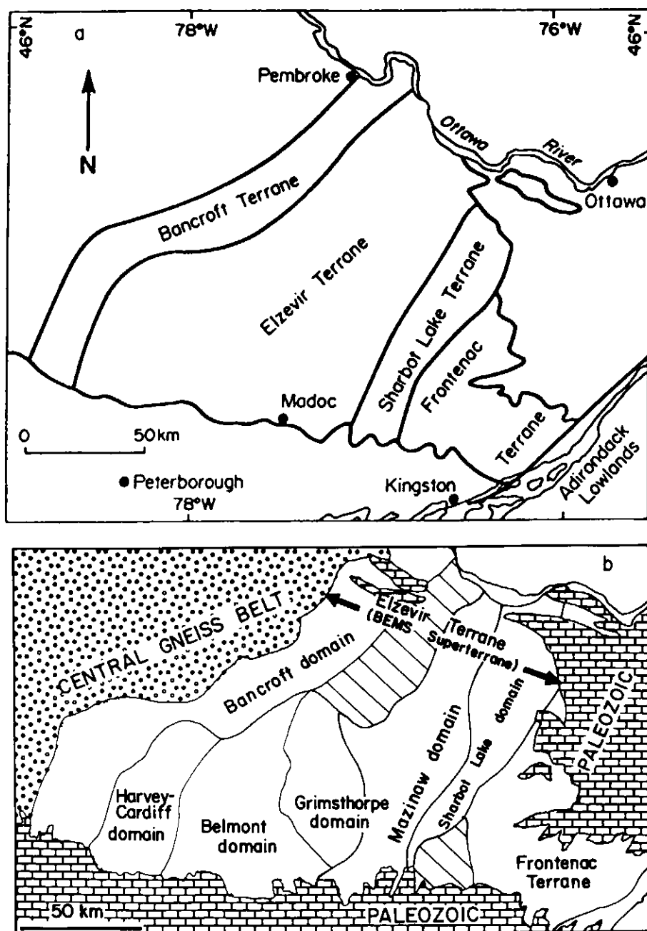
Figure 1 (A) Terrane subdivision of the Central Metasedimentary Belt as proposed by Moore (1982). (B) Proposed terrane subdivision of the Central Metasedimentary Belt (after Easton 1992). Diagonally hatched areas are not easily assigned to any existing domain. (BEMS = Bancroft-Elzevir-Mazinaw-Sharbot Lake.)
