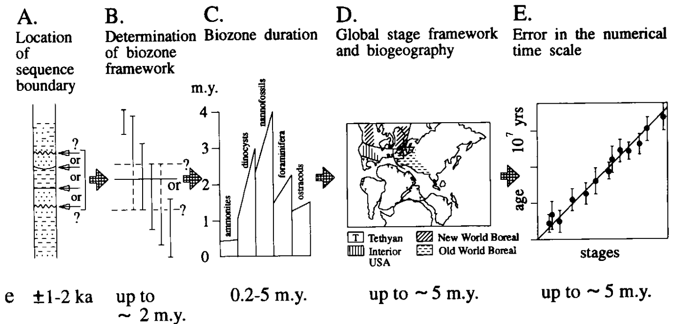
Figure 7 Steps in the correlation and dating of stratigraphic events. e=typical range of error associated with each step. (A) In the case of the sequence framework, location of sequence boundaries may not be a simple matter, but depends on interpretation of the rock record using sequence principles. (B) Assignment of the boundary event to the biozone framework. An incomplete record of preserved taxa (almost always the case) may lead to ambiguity in the placement of biozone boundaries. (C) The precision of biozone correlation depends on biozone duration. Shown here is a simplification of Cox's (1990) summary of the duration of zones in Jurassic sediments of the North Sea Basin. (D) The building of a global stage framework is fundamental to the development of a global time scale. However, global correlation is hampered by faunal provincialism. Shown here is a simplification of the faunal provinces of Cretaceous ammonites, shown on a mid-Cretaceous plate-tectonic reconstruction. Based on Kennedy and Cobban (1977) and Kauffman (1984). (E) The assignment of numerical ages to stage boundaries and other stratigraphic events contains inherent experimental error and also the error involved in the original correlation of the datable horizon(s) to the stratigraphic event in question. Diagrams of this type are a standard feature of any discussion of the global time scale (e.g., Haq et al. , 1988; Harland et al. , 1990). The establishment of a global biostratigraphically-based sequence framework involves the accumulation of uncertainty over steps A to D. Potential error may be reduced by the application of radiometric, magnetostratigraphic or chemostratigraphic techniques which, nonetheless, contain their own inherent uncertainties (step E).
