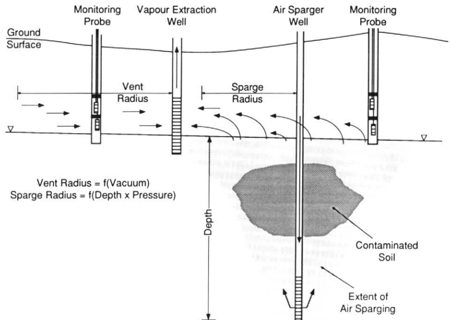
Figure 21 Typical air-sparging system.
