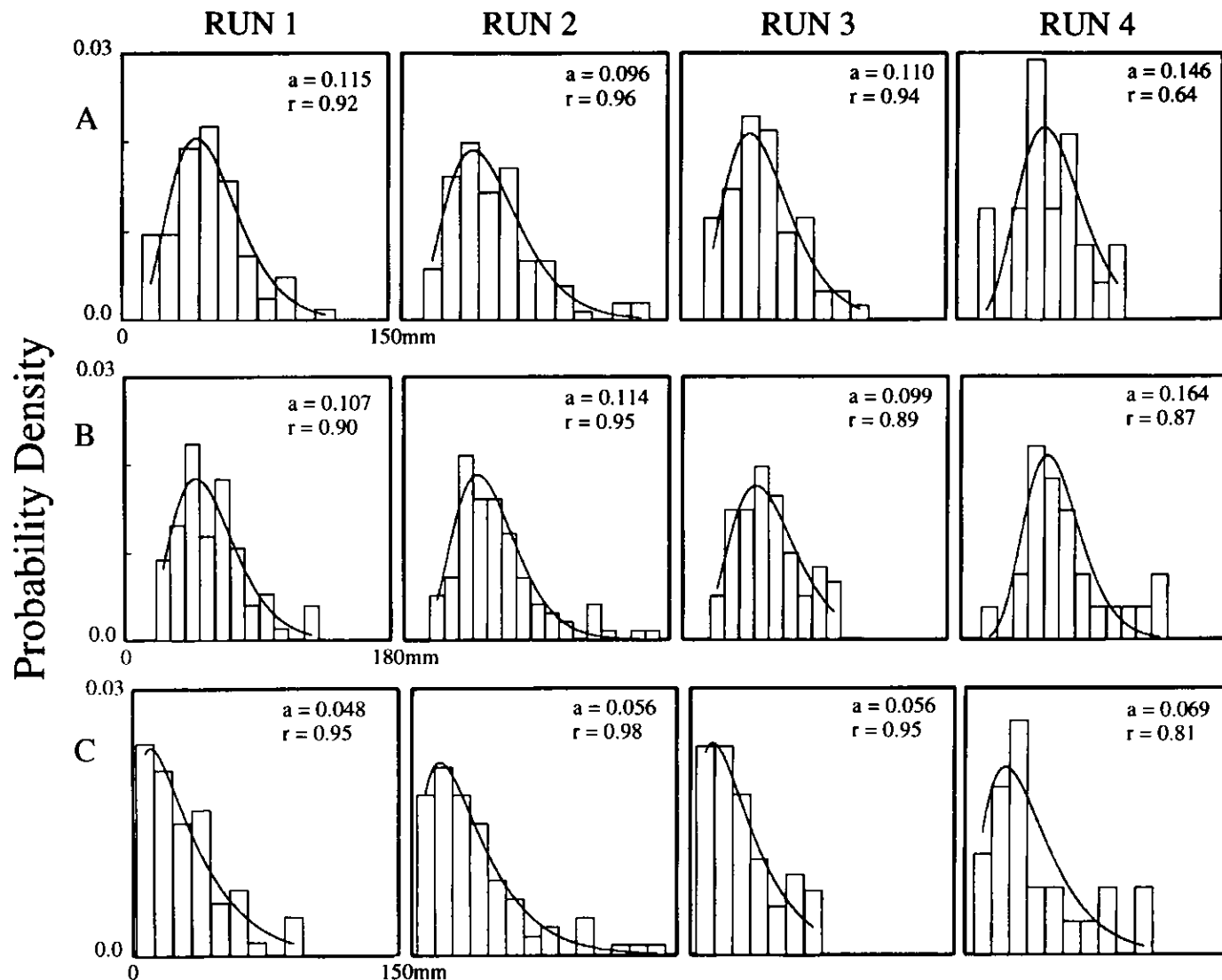
Figure 5 Histograms of dune height (A) and dune trough elevation relative to the upper reference datum (B) and mean bed-height datum (C) for all runs, with fitted gamma functions.
