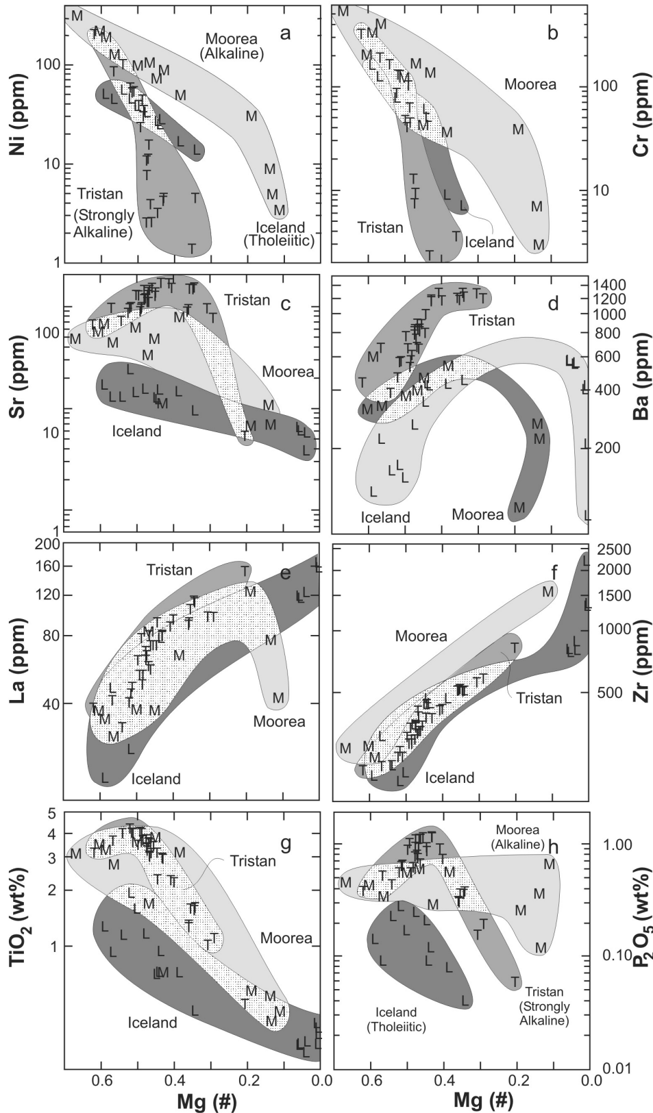
Figure 13. Plots of selected trace elements (ppm) and major element oxides (wt. %) versus the differentiation indicator Mg# (= Mg/(Mg + (0.9*Fe total )) atomic) in three suites of oceanic island basalts. Tristan da Cunha (T) represents a strongly alkaline suite, Moorea Society Islands, (M) a moderately alkaline suite and Iceland (L) a tholeiitic suite. Note concentrations on the Y axis are on a log scale.
