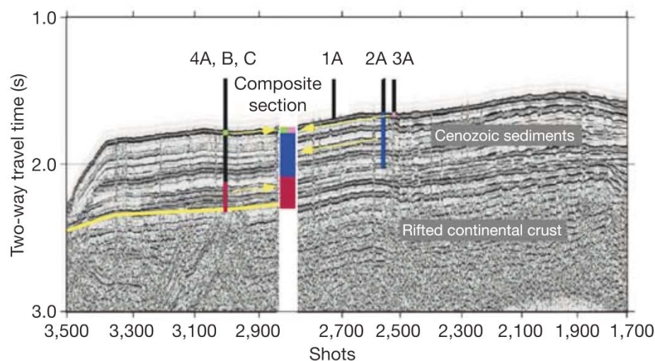
Figure 4. Seismic reflection line showing the ACEX drill sites and the composite section. Figure from Moran et al. (2006); seismic data from Joket et al. (1992).
