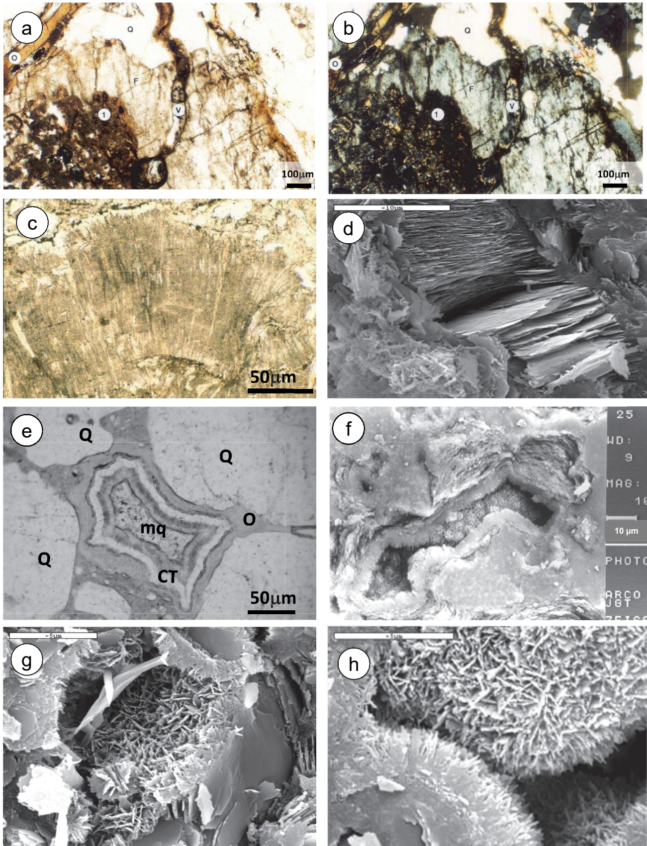
Figure 3. Mineralogical characterization of the Bleeding Stone and Ochre Granite. a) and b) Thin section photomicrographs (plane- and cross-polarized light, respectively) of a level in the middle of the palaeoweathered zone, Ochre Granite. Feldspar (F) is weathered and cracks are filled mainly by opal-CT (O) and clays (1); V= residual void space; Q = quartz; c) thin section photomicrograph of kaolinite; d) SEM photomicrograph of kaolinite; e) thin section photomicrograph of opal-CT (O) lining a cavity; CT= opal-CT lepispheres; mq = chalcedony microcrystalline quartz; Q = quartz; f) SEM photomicrograph of opal-CT lepispheres (spherical rosettes of authigenic silica formed during low-temperature diagenesis) lining a cavity; g) SEM photomicrograph of opal-CT and 1:1 phyllosilicates; h) SEM photomicrograph of opal-CT lepispheres.
