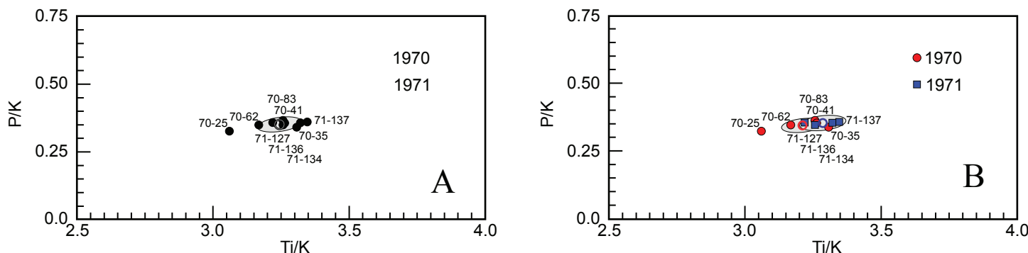
Figure 3. Conserved element plots for the 1970–1971 Mauna Ulu lava flows. Plotted are two ratios formed from three elements likely to be conserved in basaltic systems: P/K and Ti/K. Mean values are indicated by open circles. The shaded ellipses represent the expected variation in location of the mean values due to analytical uncertainty. (A) Distribution of the data points for the entire 1970–1971 data set. Several points fall outside the expected uncertainty about the mean, especially along the Ti/K axis. (B) Distribution of data points grouped by date of eruption. The 1971 data points fall within their uncertainty ellipse, whereas two of the 1970 data points (70-25 and 70-35) do not.
