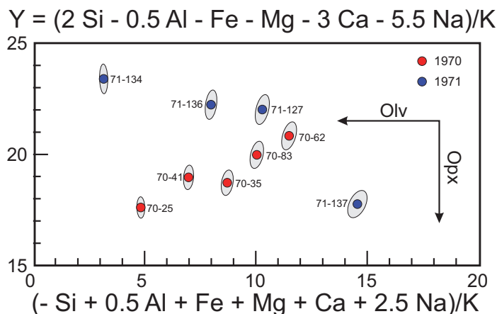
Figure 11. Pearce element ratio diagram that contrasts the pattern expected from olivine fractionation with the pattern expected from orthopyroxene fractionation. One can verify that plagioclase ( \text{CaAl}_2\text{Si}_2\text{O}_8 , \text{NaAlSi}_3\text{O}_8 ) and clinopyroxene [ \text{Ca}(\text{Mg,Fe})\text{Si}_2\text{O}_6 ] would produce a zero-length vector on the diagram. The arrows point in the direction fractionation (loss from system) would distribute data points.
