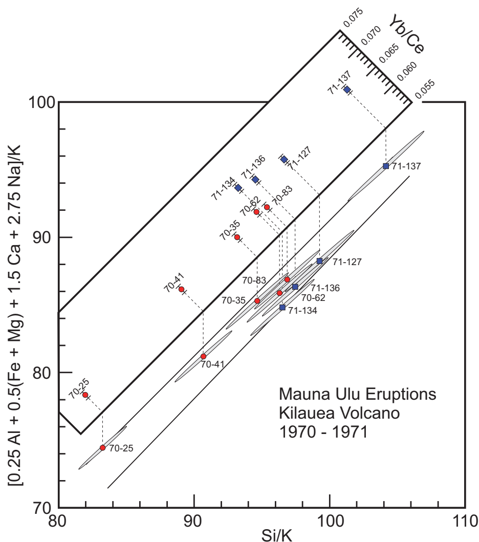
Figure 5. Same diagram as Figure 4 but with the ratios of two incompatible trace elements (Yb and Ce) projected on the diagram. The distribution of the trace element ratios distinguishes the flows erupted in 1970 from those erupted in 1971, indicating the presence of two chemical systems among the eruptive products. The shaded ellipses represent the expected variation in location of the data points due to analytical uncertainty.
