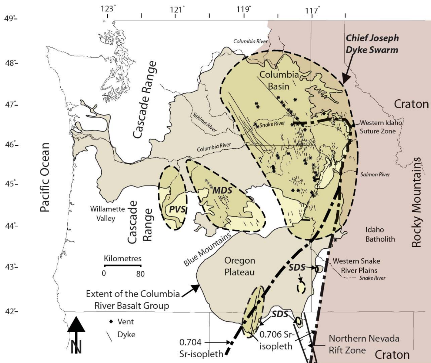
Figure 1. Location map of the Columbia River flood basalt province. This figure shows the extent of the Columbia River Basalt Group and dykes. The Columbia Basin forms the northern portion of the province and the Oregon Plateau forms the southern portion of the province south of the Blue Mountains. Geographic features include: Chief Joseph dyke swarm, Steens Basalt dyke swarms (SDS), Monument (Picture Gorge) dyke swarm (MDS) and Prineville Basalt source area (PVS). The initial mainly granitic ^{87}\text{Sr}/^{86}\text{Sr} 0.704 and 0.706 isopleths are from Pierce and Morgan (2009) and Armstrong et al. (1977). The Precambrian craton lies east of the 0.706 isopleth, oceanic accreted terranes lie west of the 0.704 isopleth, and transitional crust with cratonic affinities lies between the two. Basement rocks include the Precambrian craton of North America east of the 0.706 line, transitional crust with cratonic affinity between the 0.706 and 0.704 lines, and Paleozoic to Mesozoic oceanic accreted terranes west of the 0.704 line.
