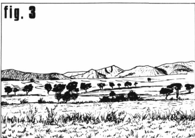
FIGURE 3. L'alvéole granodioritique de Kaap Valley et les crêtes appalachiennes des Jamestown Hills (vus du sud-est). The granodiorite basin of Kaap Valley and the Appalachian crests of Jamestown Hills (as seen from the south-east).
